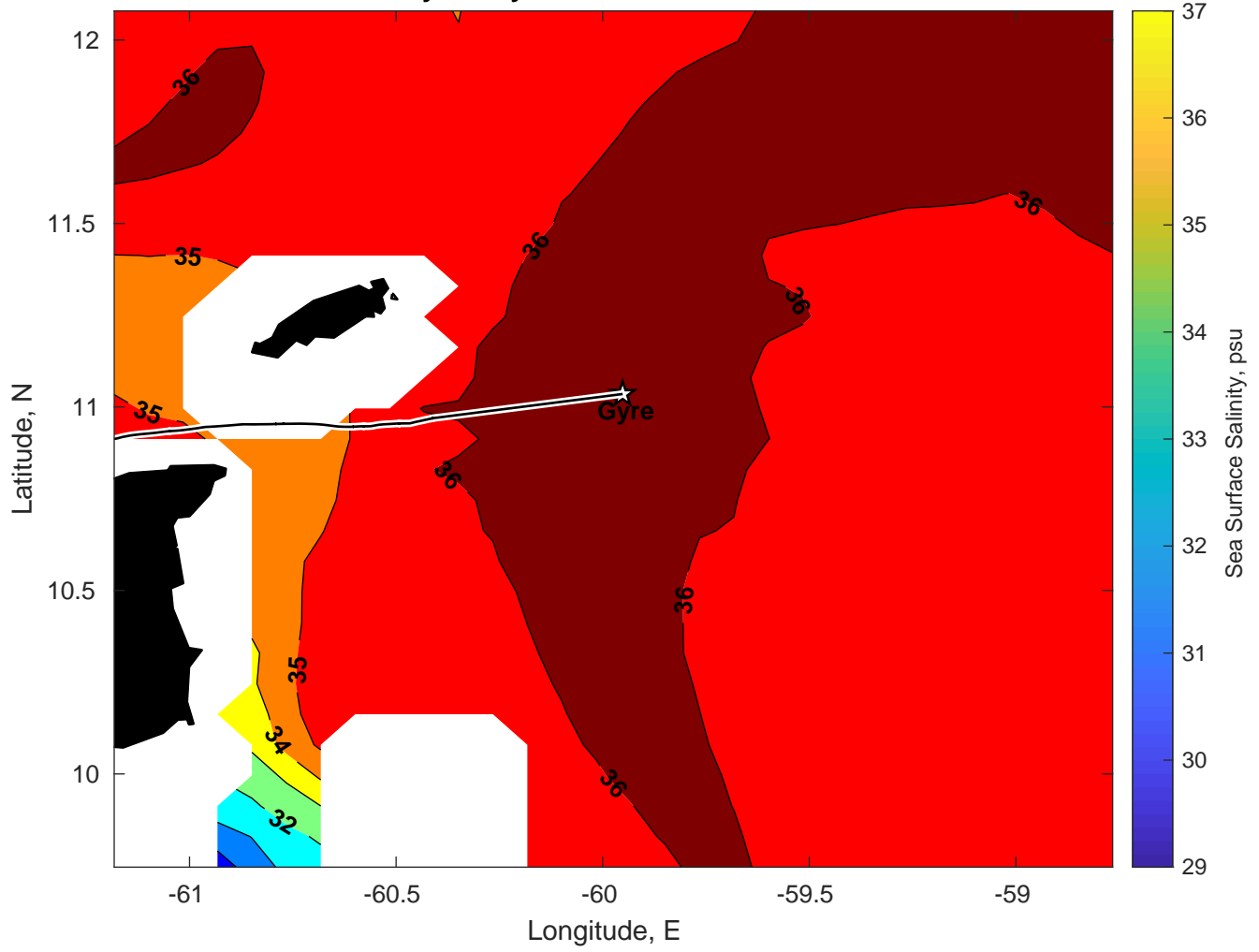
Surface Salinity for Gyre at 12-Jan-2025 00:00:00
