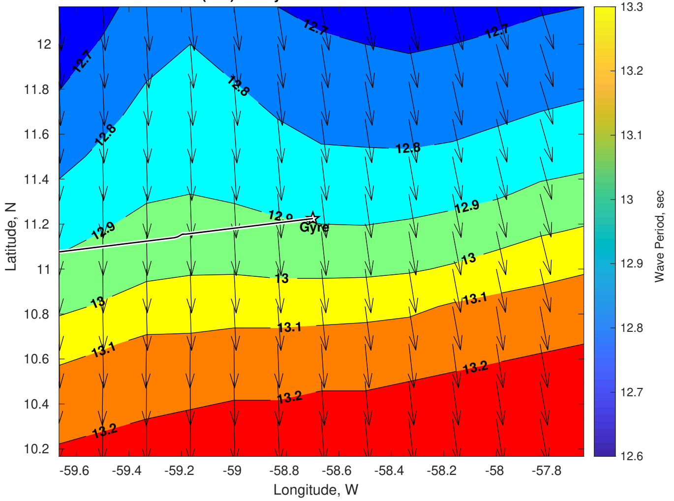
Wave Period (sec) for Gyre at 13-Jan-2025 09:00:00
