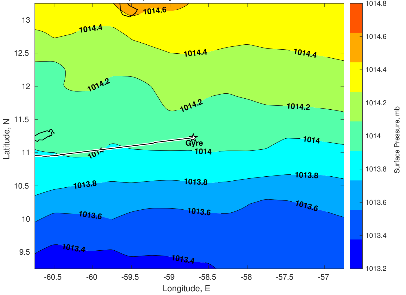
Surface Pressure (mb) for Gyre at 15-Jan-2025 00:00:00
