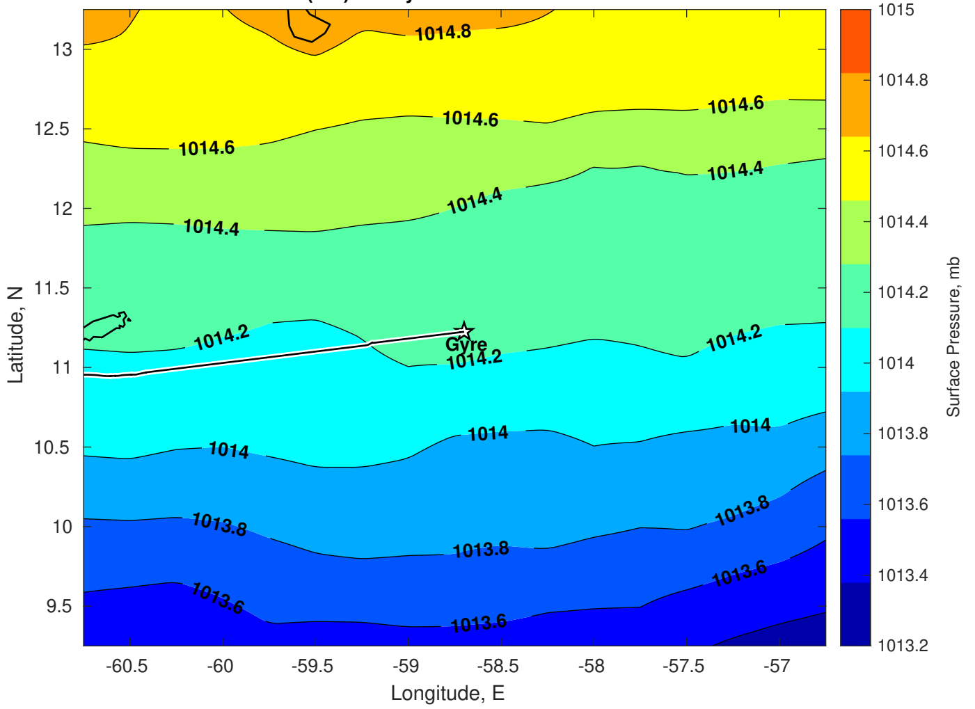
Surface Pressure (mb) for Gyre at 14-Jan-2025 00:00:00
