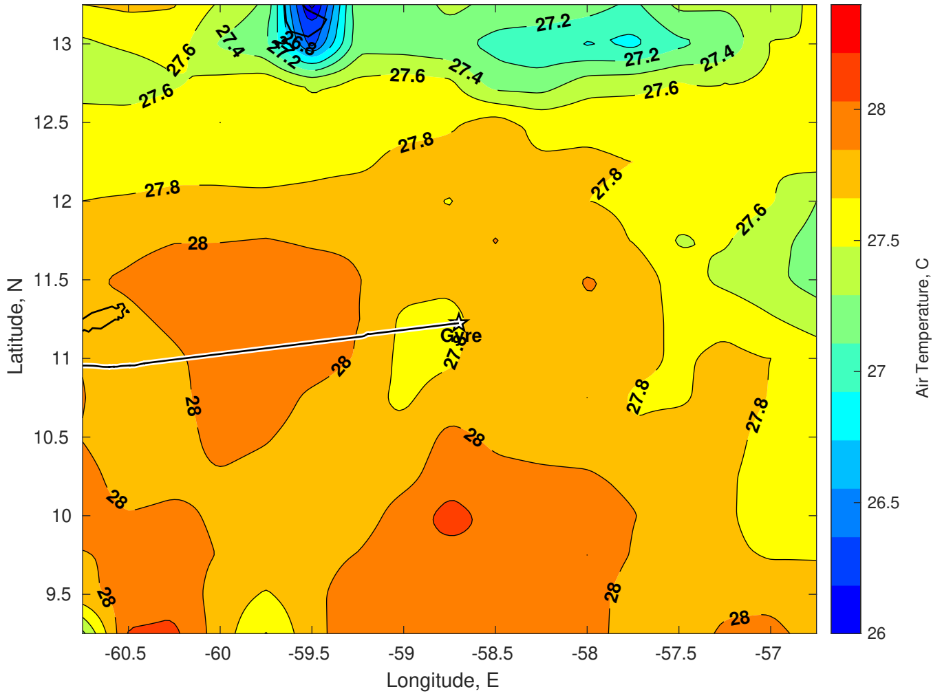
Air Temperature (C) for Gyre at 13-Jan-2025
