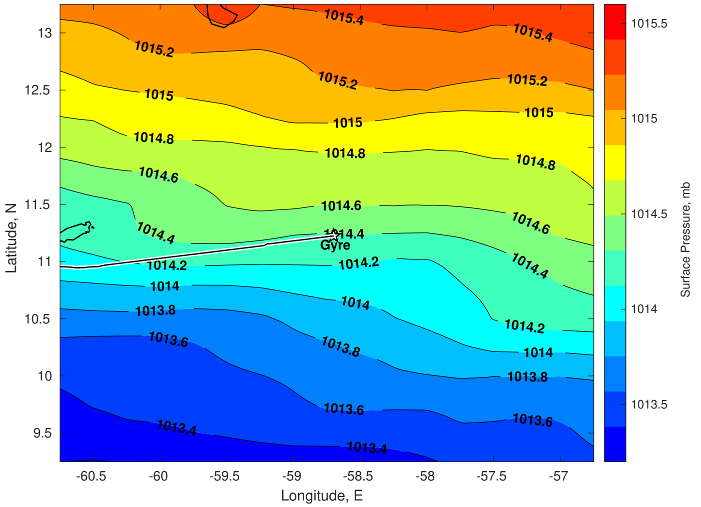
Surface Pressure (mb) for Gyre at 13-Jan-2025 00:00:00
