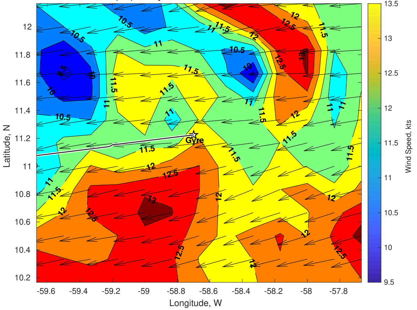
Winds (kts) for Gyre at 13-Jan-2025 09:00:00
