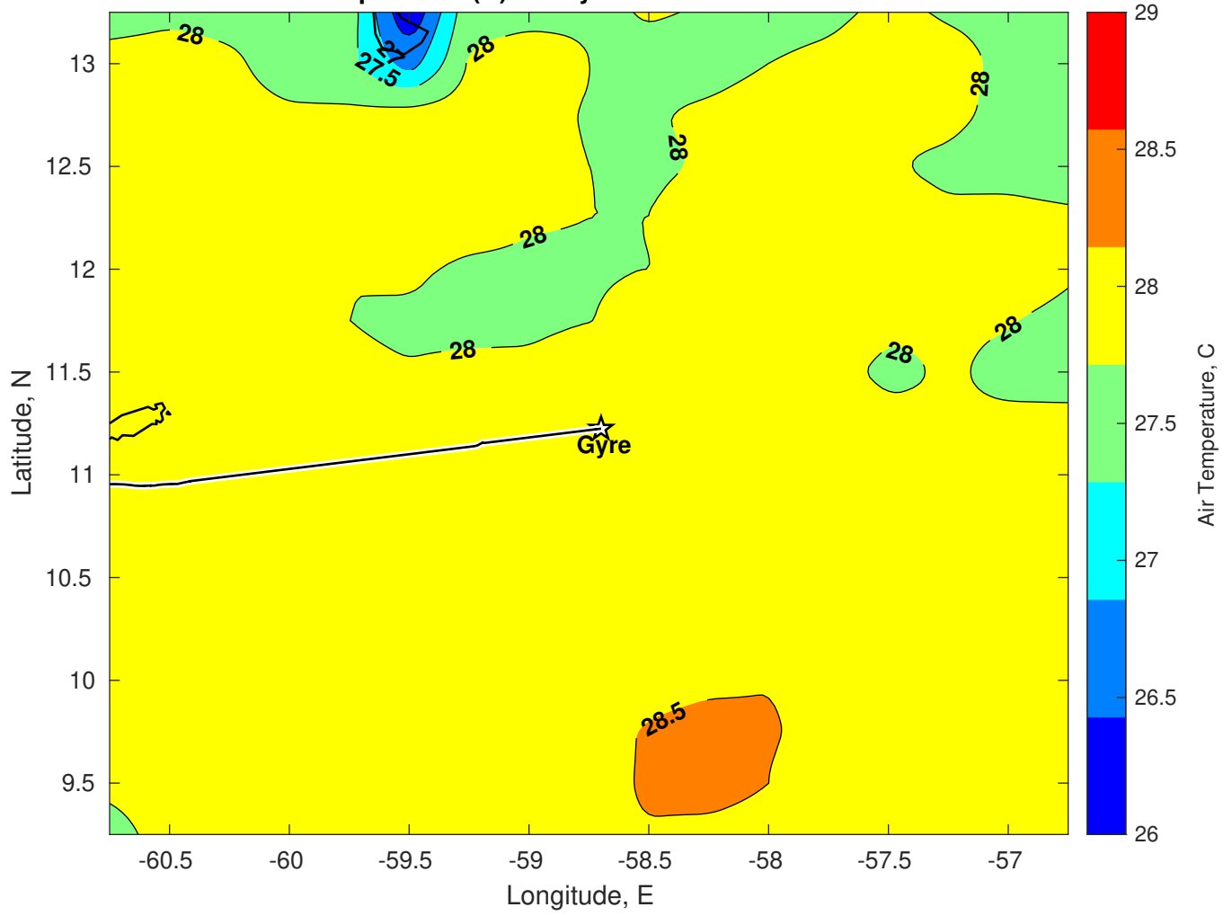
Air Temperature (C) for Gyre at 13-Jan-2025
