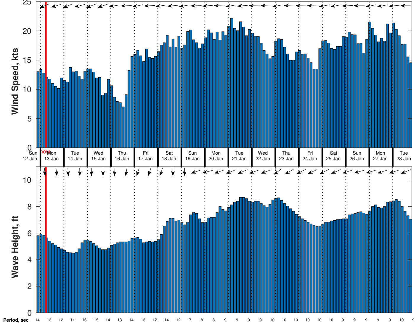
Wind & Wave Forecast for Gyre from 12-Jan-2025 20:00:00 to 28-Jan-2025 20:00:00
