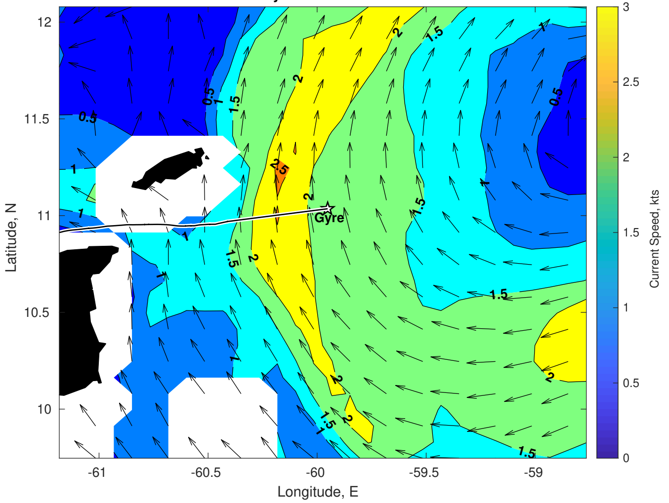
Surface Currents for Gyre at 12-Jan-2025 00:00:00
