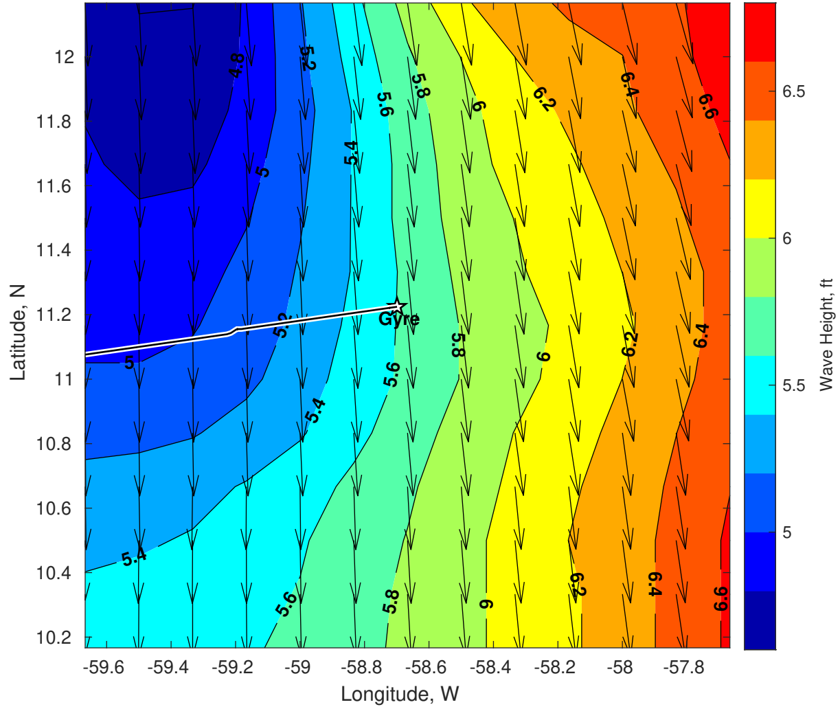
Wave Height (ft) for Gyre at 13-Jan-2025 09:00:00
