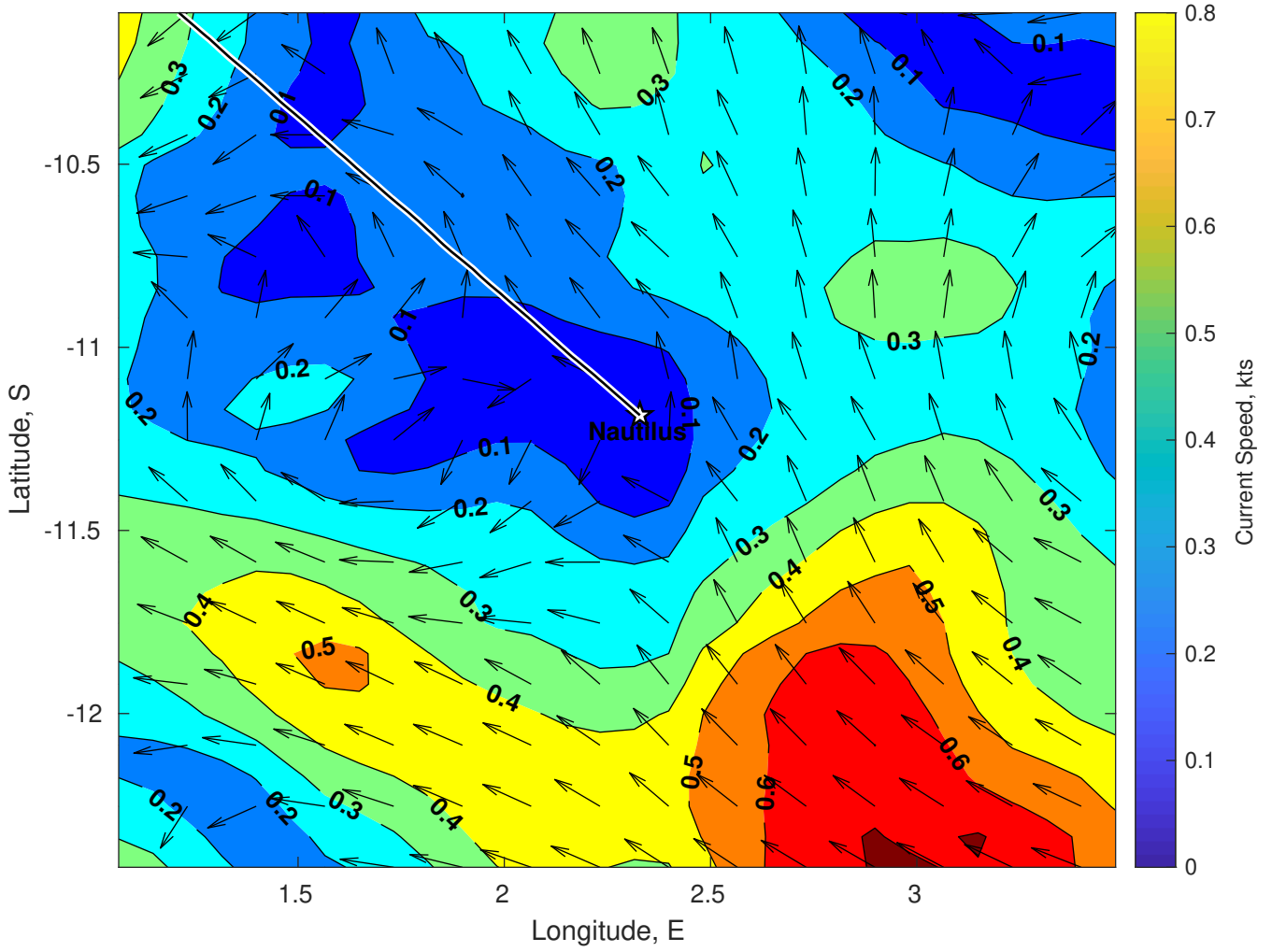
Surface Currents for Nautilus at 12-Jan-2025 00:00:00
