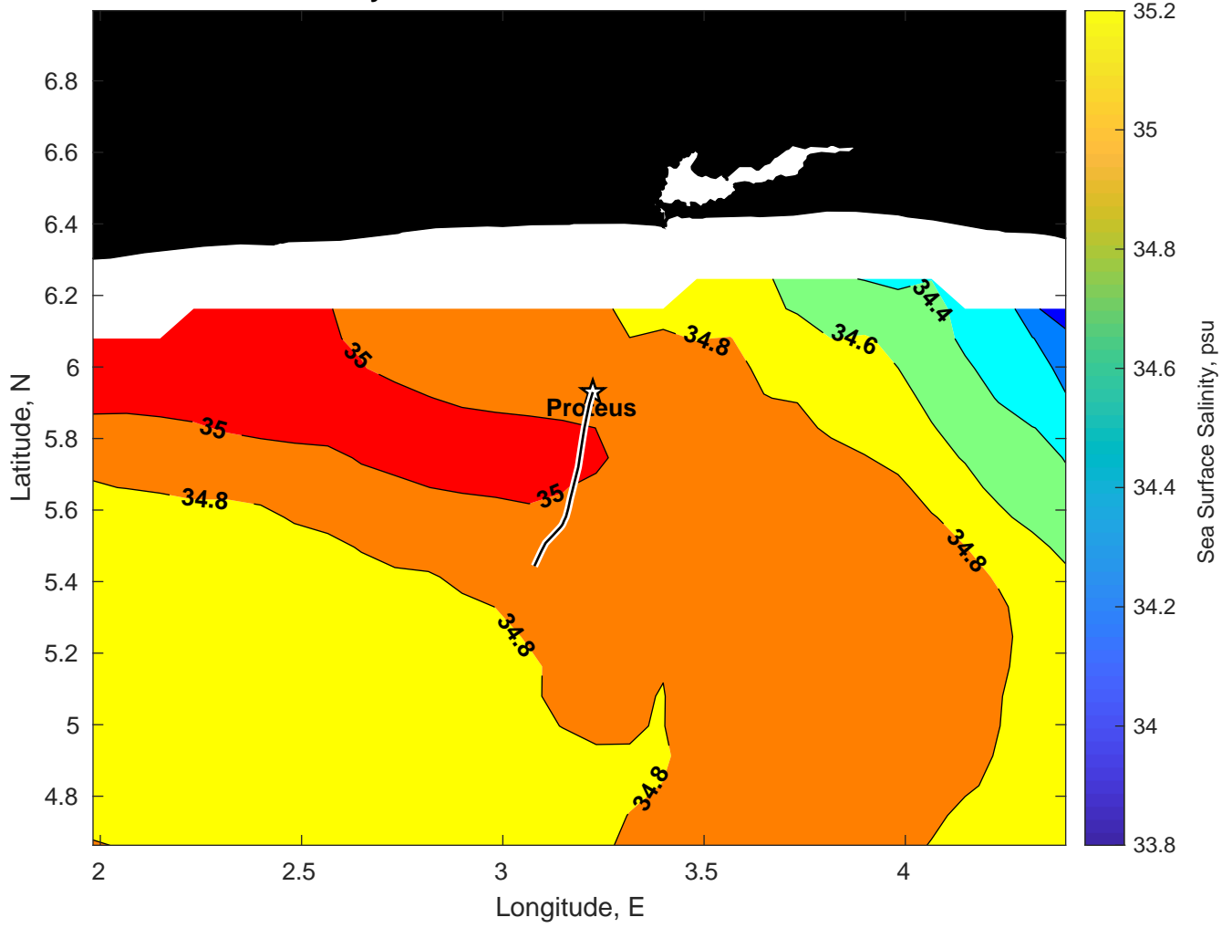
Surface Salinity for Proteus at 12-Jan-2025 00:00:00
