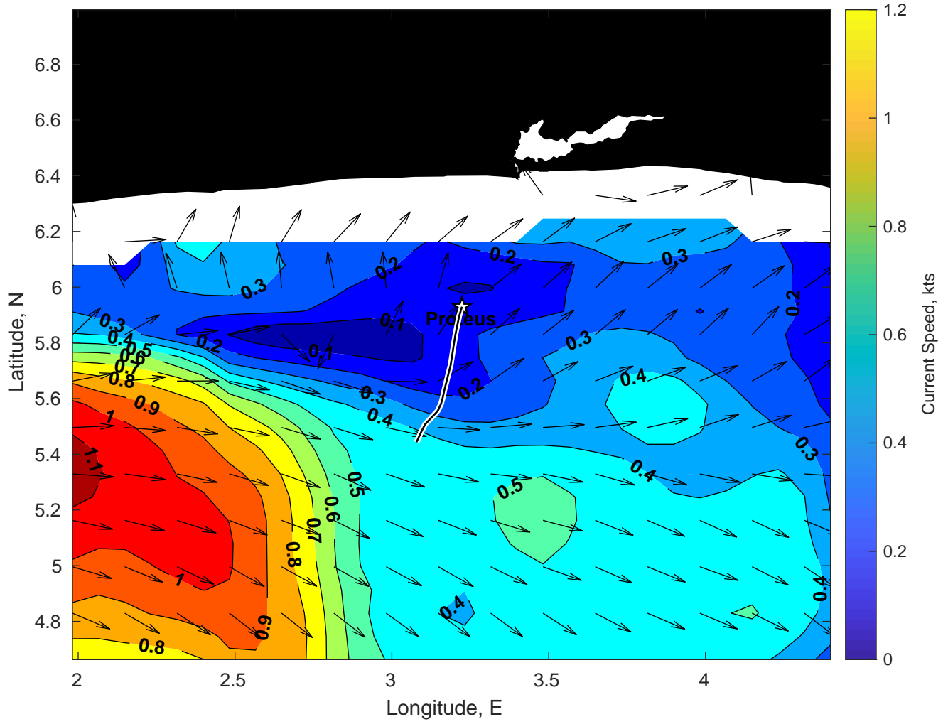
Surface Currents for Proteus at 12-Jan-2025 00:00:00
