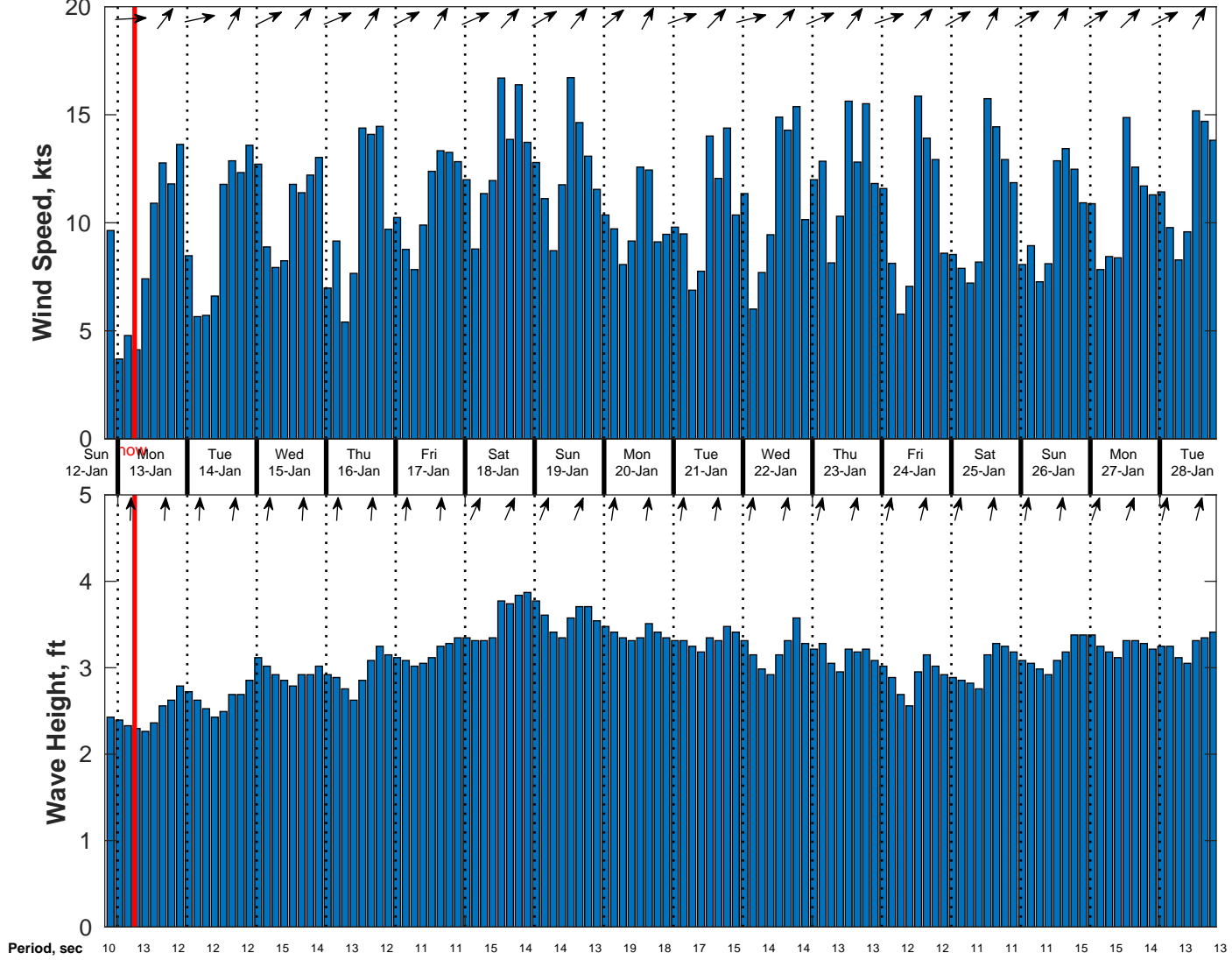
Wind & Wave Forecast for Proteus from 12-Jan-2025 20:00:00 to 28-Jan-2025 20:00:00
