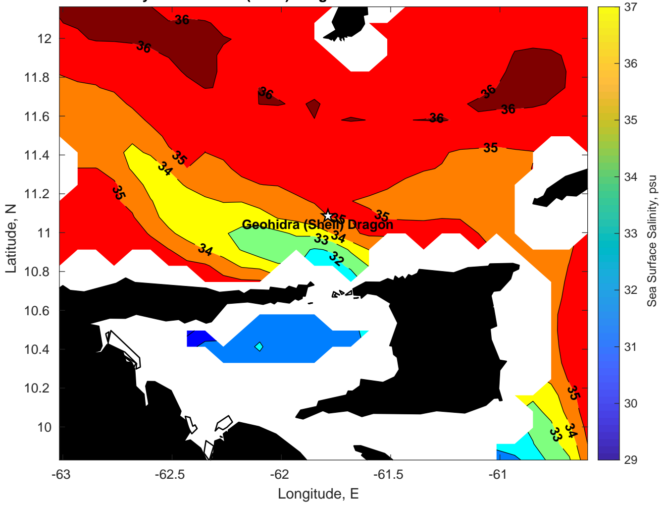
Surface Salinity for Geohidra (Shell) Dragon at 13-Jan-2025 00:00:00
