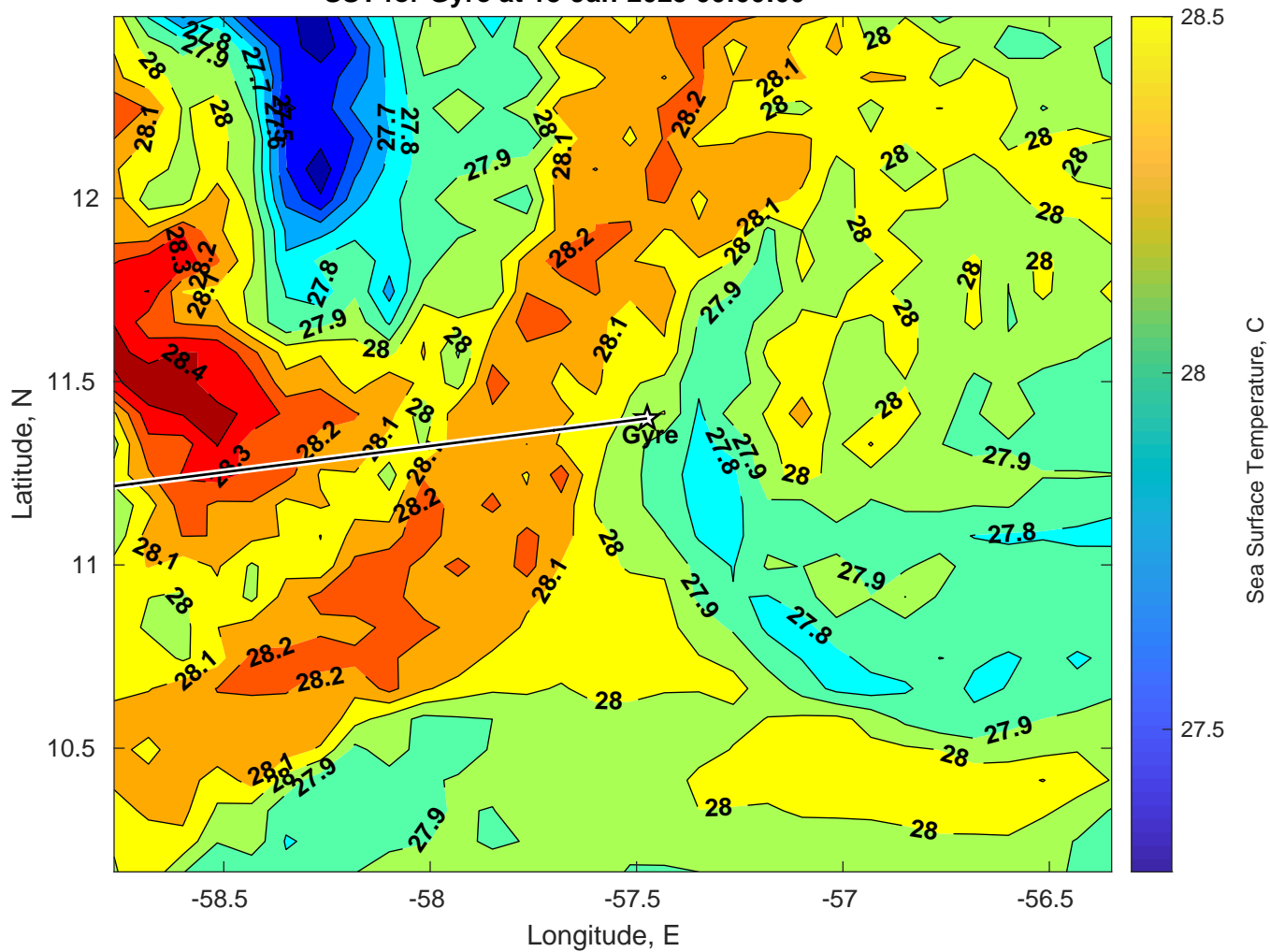
SST for Gyre at 13-Jan-2025 00:00:00
