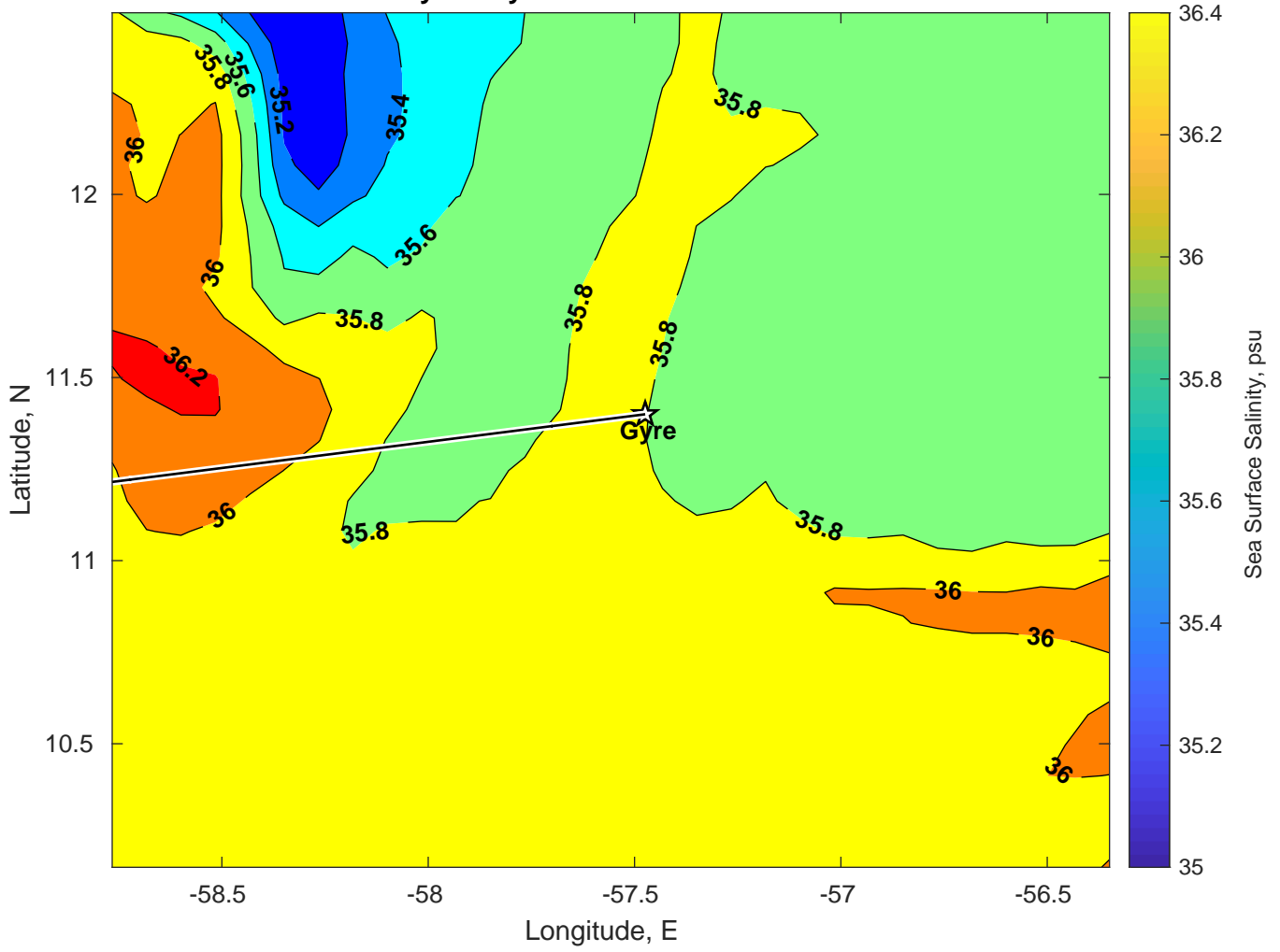
Surface Salinity for Gyre at 13-Jan-2025 00:00:00
