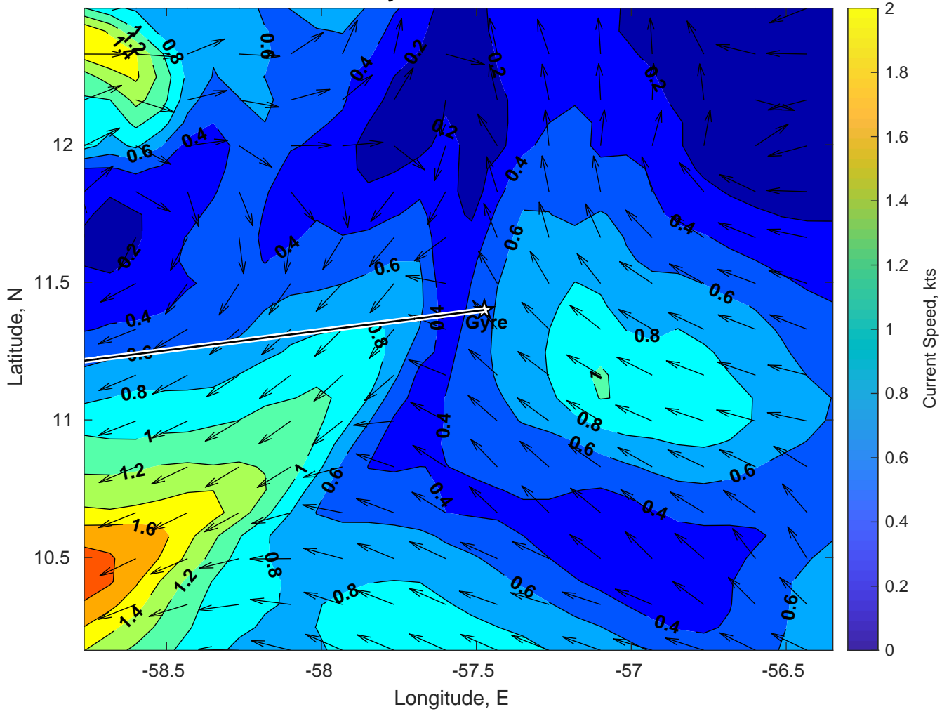
Surface Currents for Gyre at 13-Jan-2025 00:00:00
