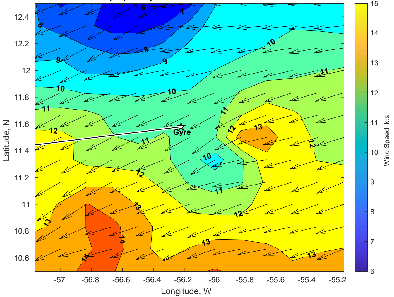
Winds (kts) for Gyre at 14-Jan-2025 09:00:00
