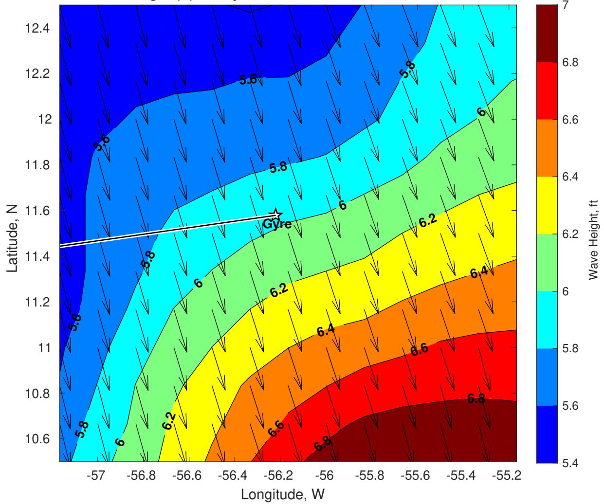
Wave Height (ft) for Gyre at 14-Jan-2025 09:00:00
