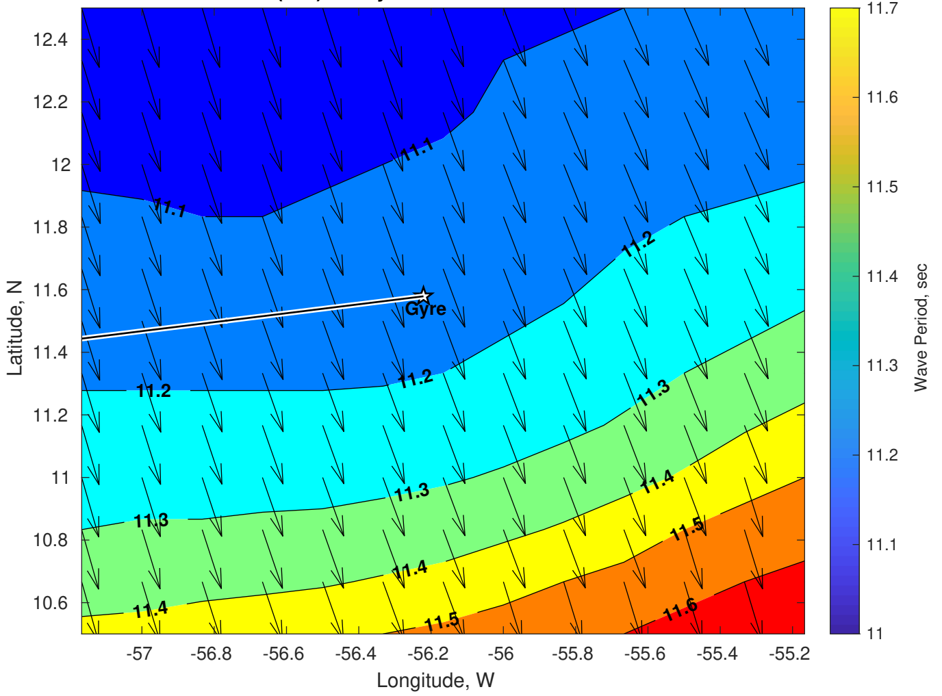
Wave Period (sec) for Gyre at 14-Jan-2025 09:00:00
