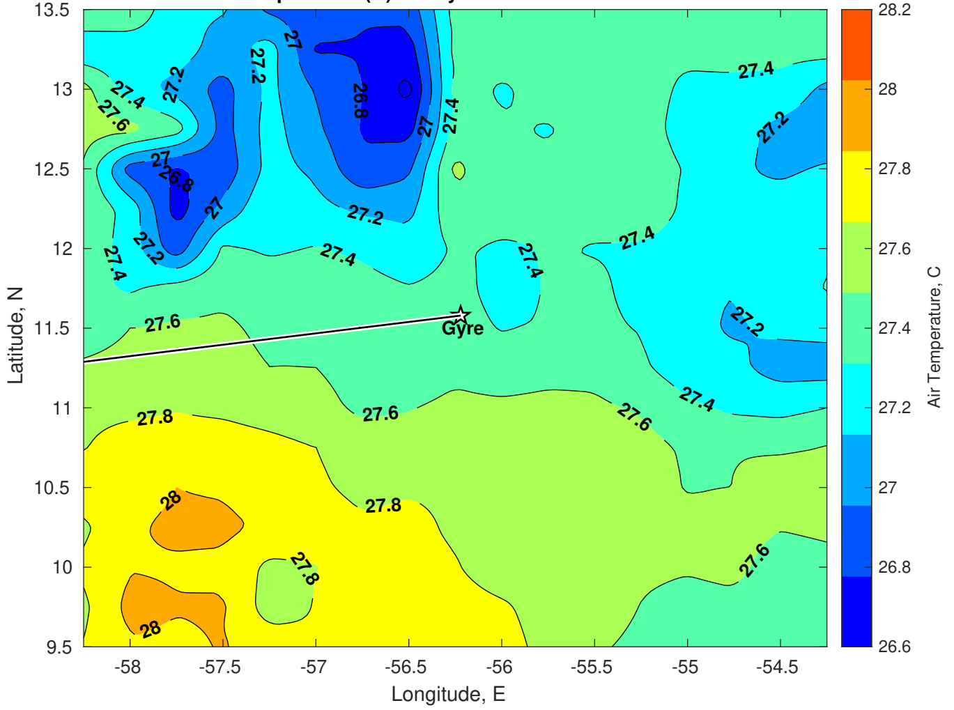
Air Temperature (C) for Gyre at 14-Jan-2025
