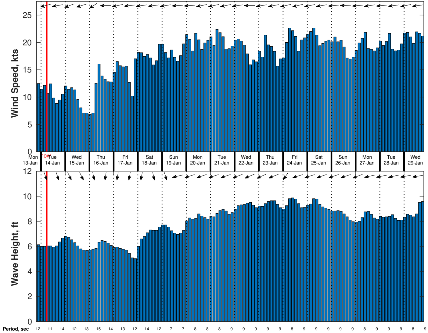
Wind & Wave Forecast for Gyre from 13-Jan-2025 20:00:00 to 29-Jan-2025 20:00:00
