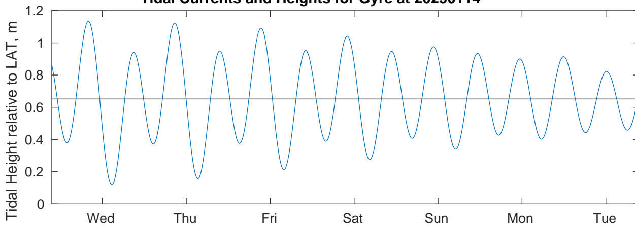
Tidal Currents and Heights for Gyre at 20250114
