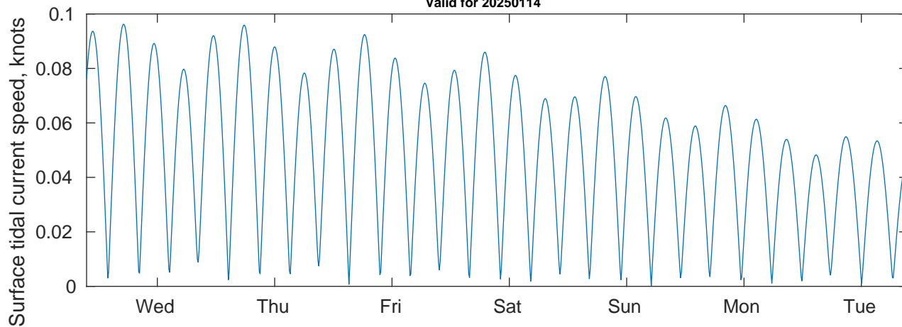
Tidal Currents and Heights for Gyre at 20250114
