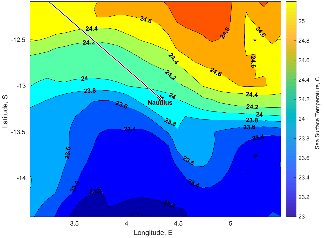
SST for Nautilus at 13-Jan-2025 00:00:00
