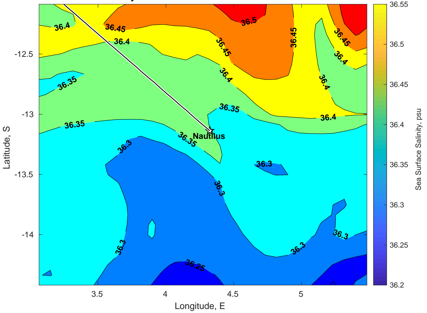
Surface Salinity for Nautilus at 13-Jan-2025 00:00:00
