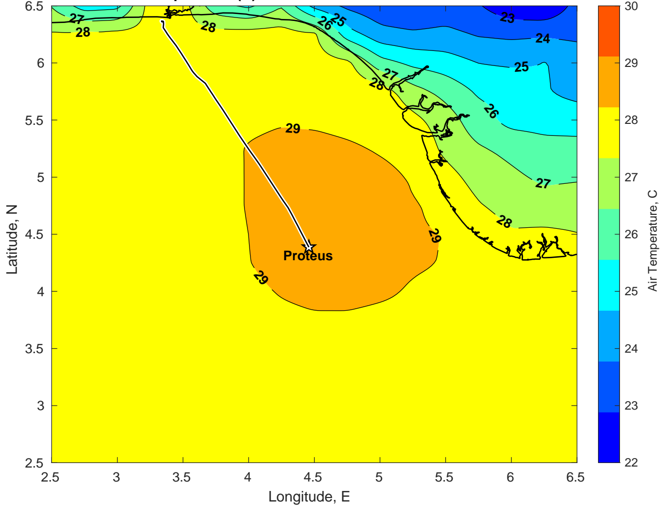
Air Temperature (C) for Proteus at 14-Jan-2025
