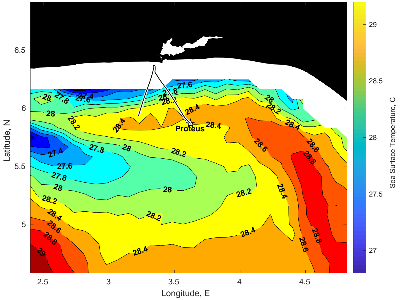
SST for Proteus at 13-Jan-2025 00:00:00
