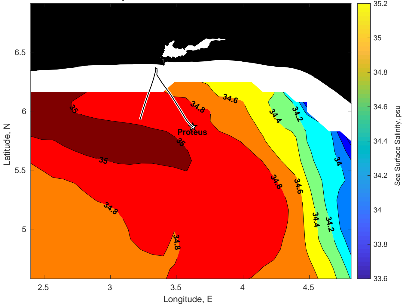
Surface Salinity for Proteus at 13-Jan-2025 00:00:00
