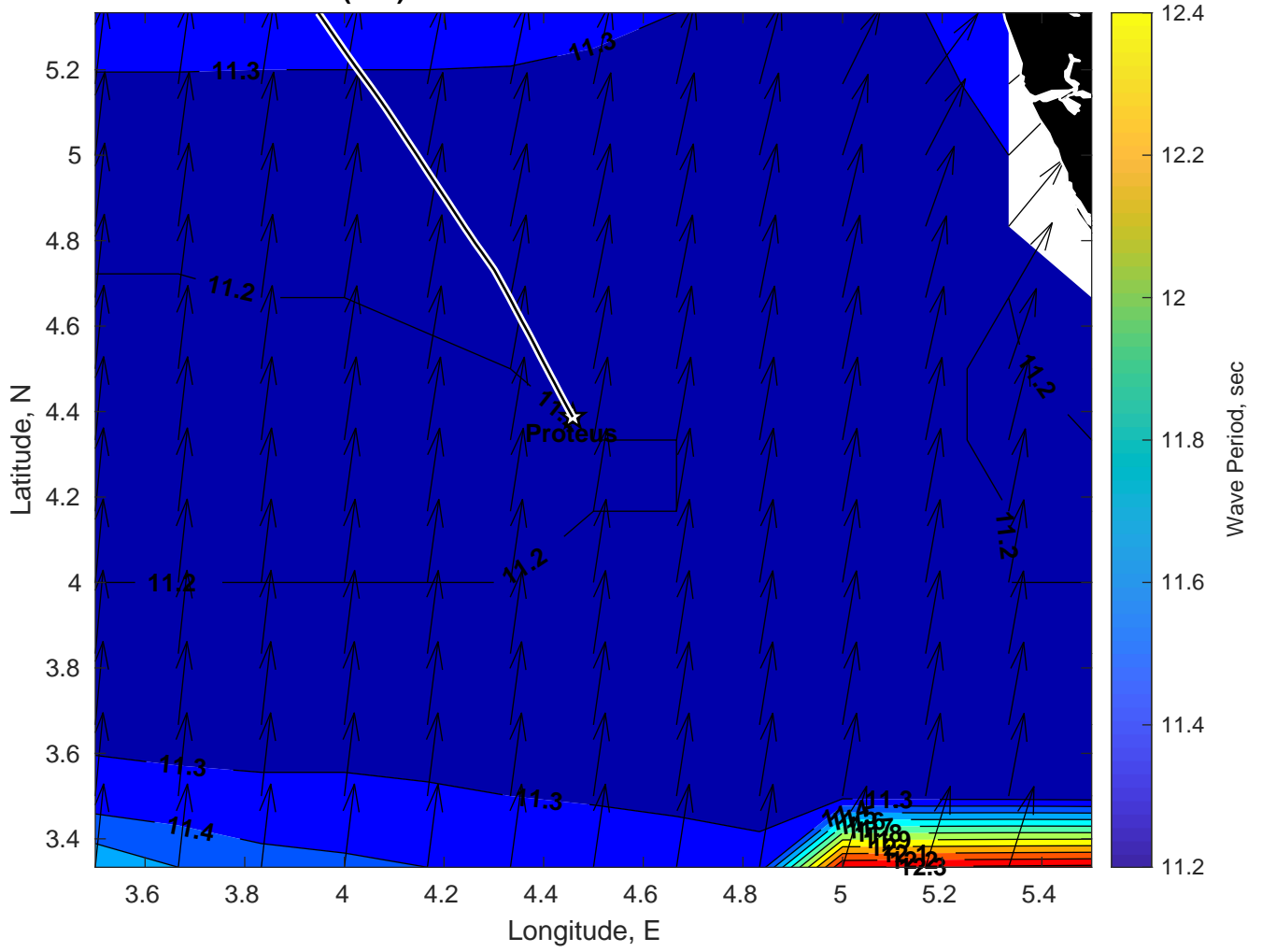
Wave Period (sec) for Proteus at 14-Jan-2025 09:00:00
