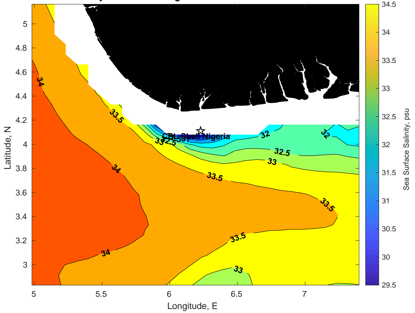
Surface Salinity for CSL Shell Nigeria at 14-Jan-2025 00:00:00
