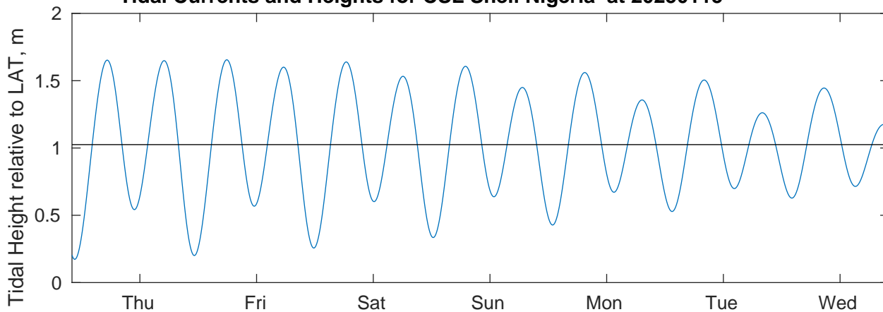
Tidal Currents and Heights for CSL Shell Nigeria at 20250115
