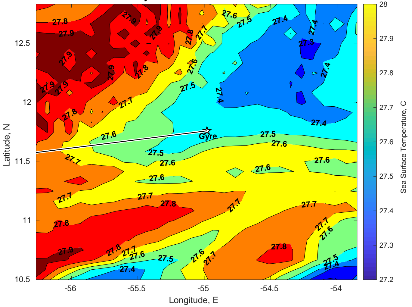
SST for Gyre at 14-Jan-2025 00:00:00
