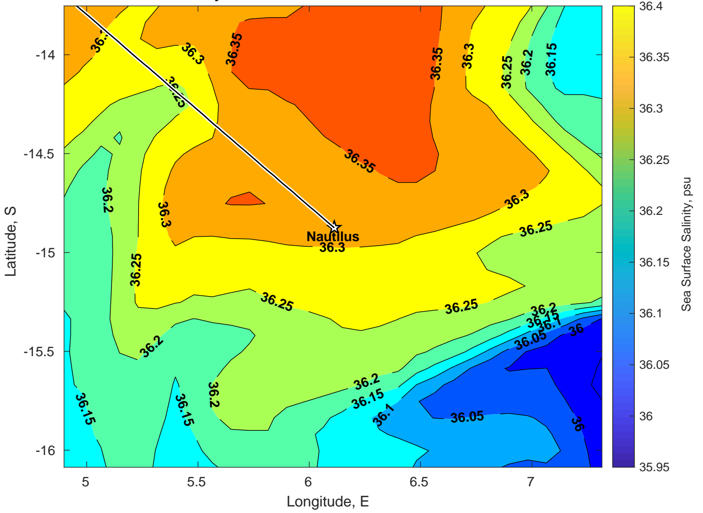
Surface Salinity for Nautilus at 14-Jan-2025 00:00:00
