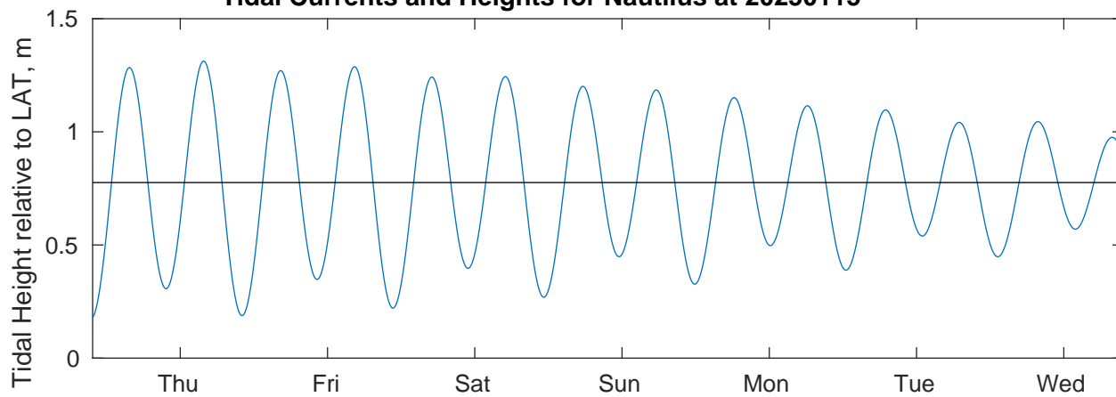
Tidal Currents and Heights for Nautilus at 20250115
