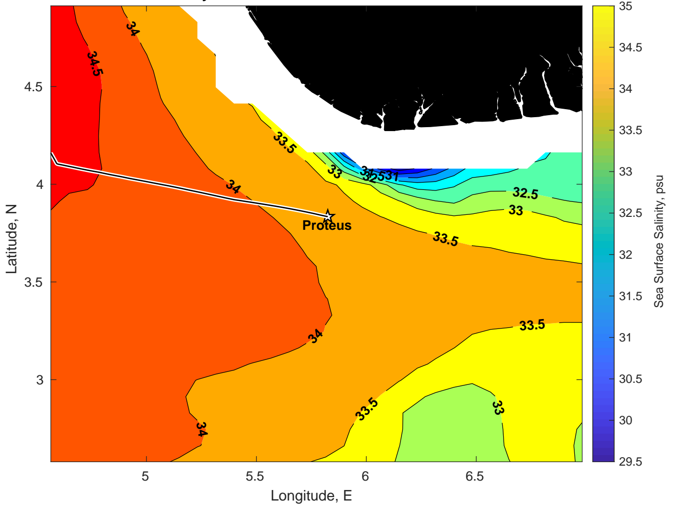
Surface Salinity for Proteus at 14-Jan-2025 00:00:00
