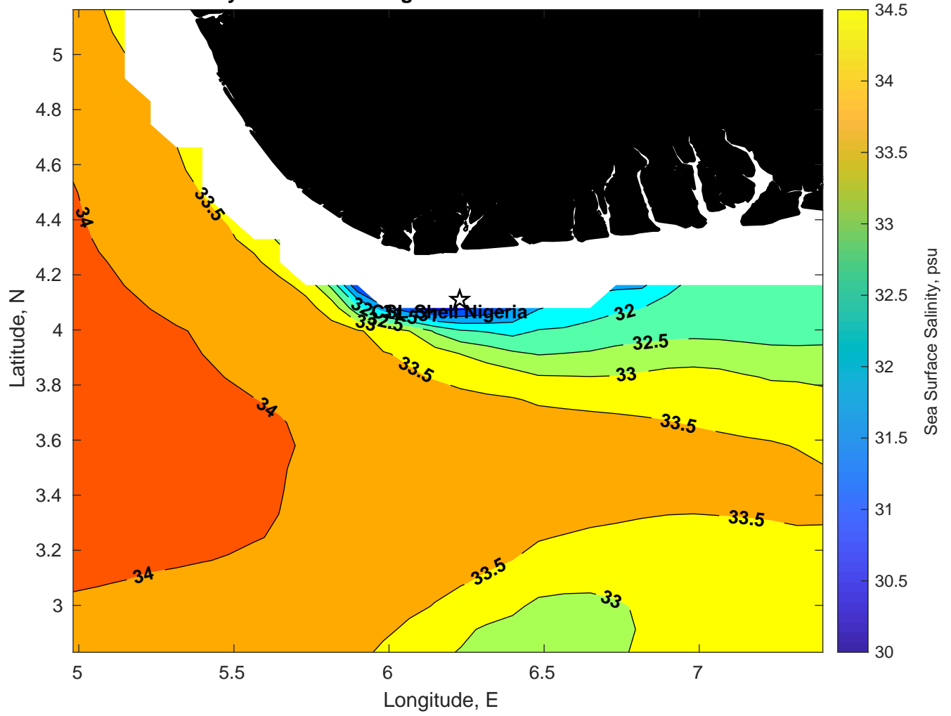
Surface Salinity for CSL Shell Nigeria at 15-Jan-2025 00:00:00
