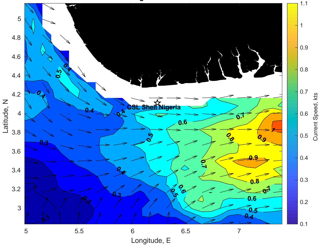
Surface Currents for CSL Shell Nigeria at 15-Jan-2025 00:00:00
