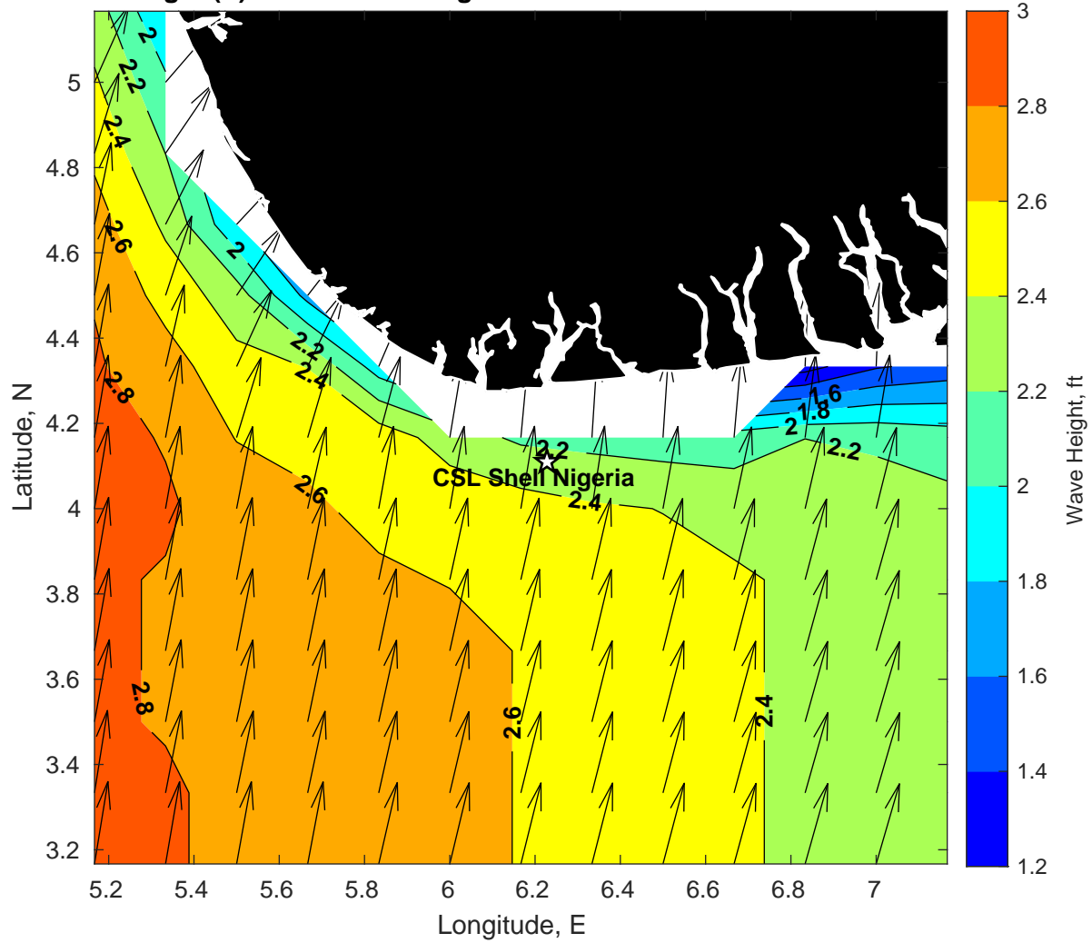
Wave Height (ft) for CSL Shell Nigeria at 16-Jan-2025 09:00:00
