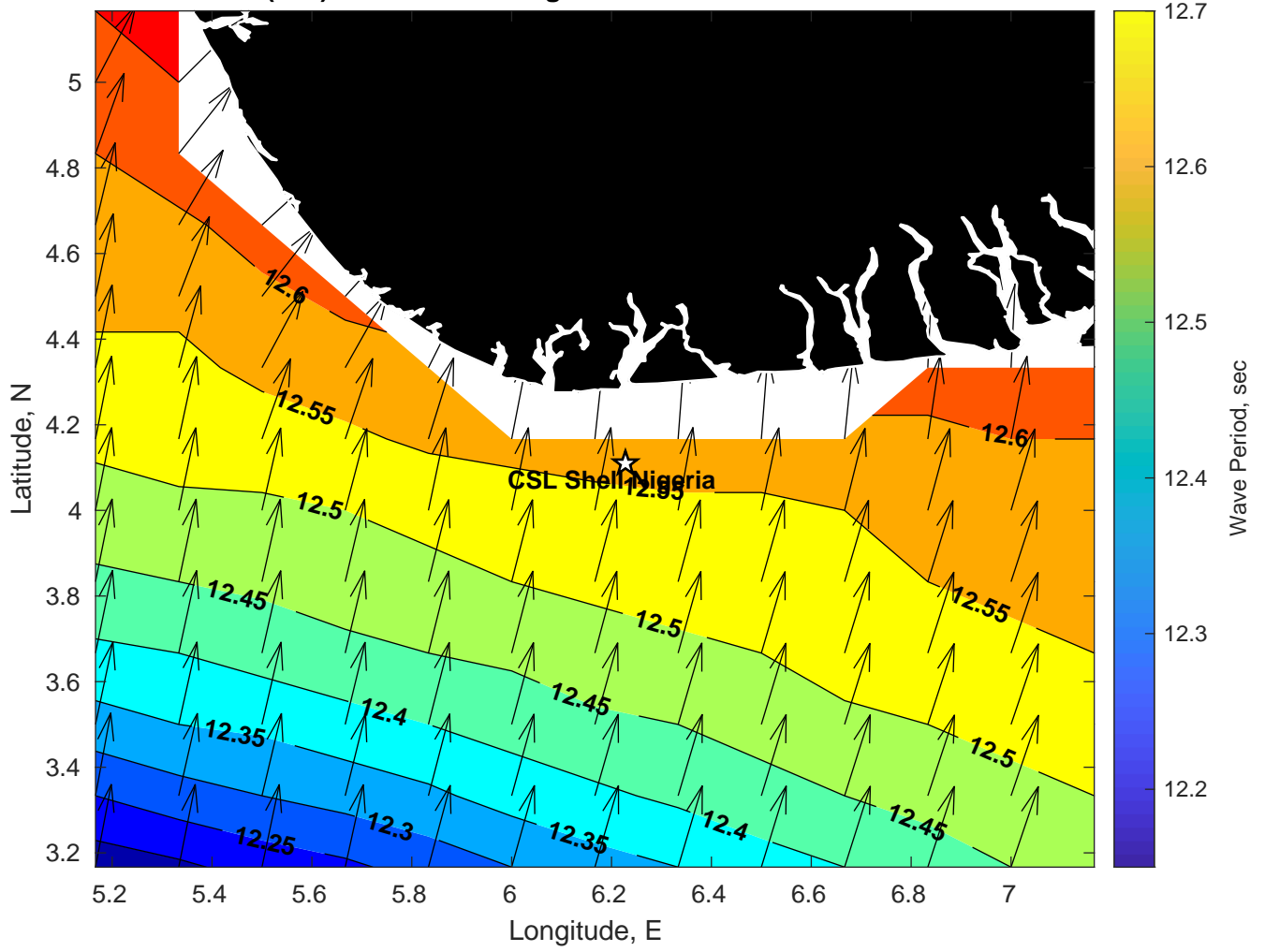
Wave Period (sec) for CSL Shell Nigeria at 16-Jan-2025 09:00:00
