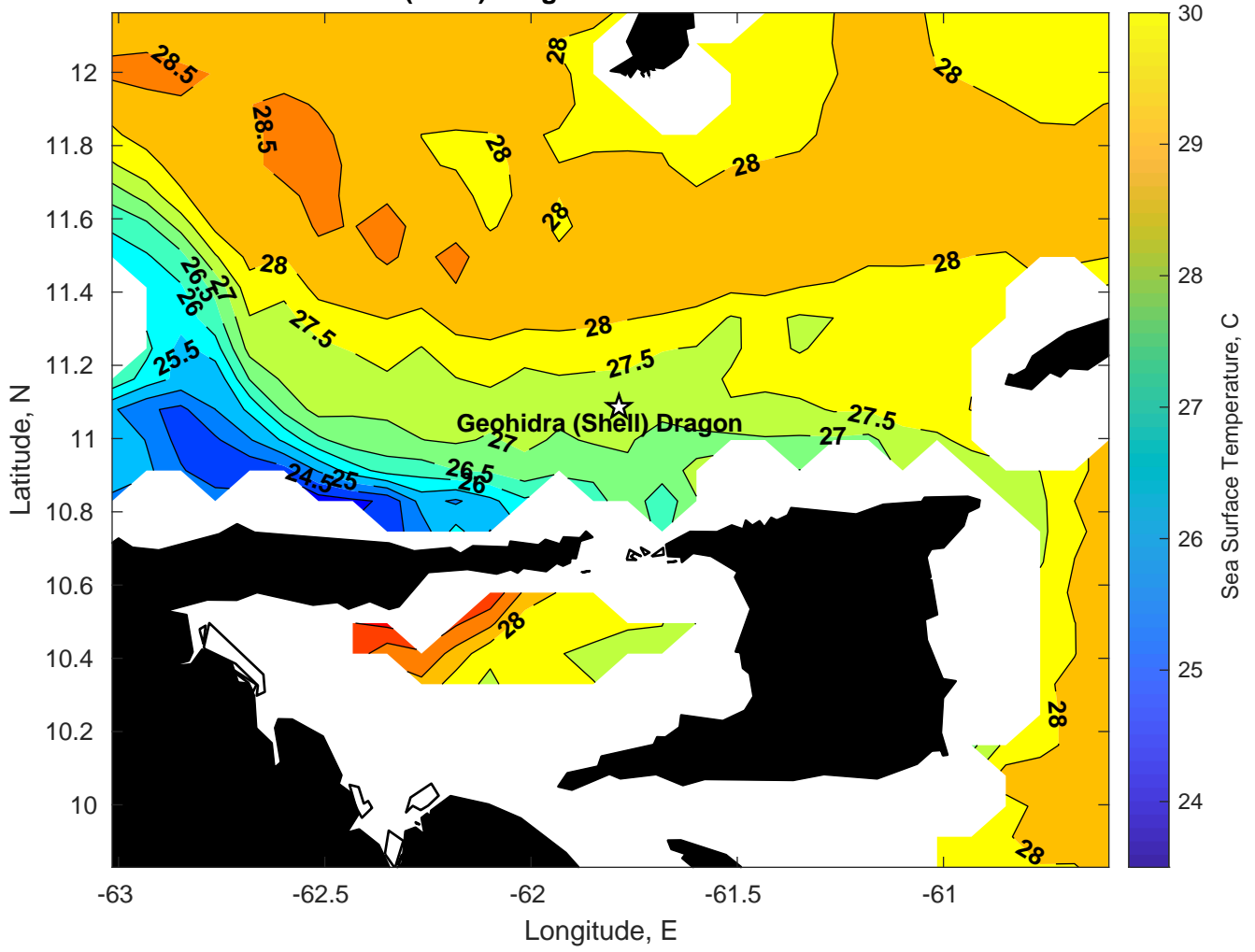
SST for Geohidra (Shell) Dragon at 15-Jan-2025 00:00:00
