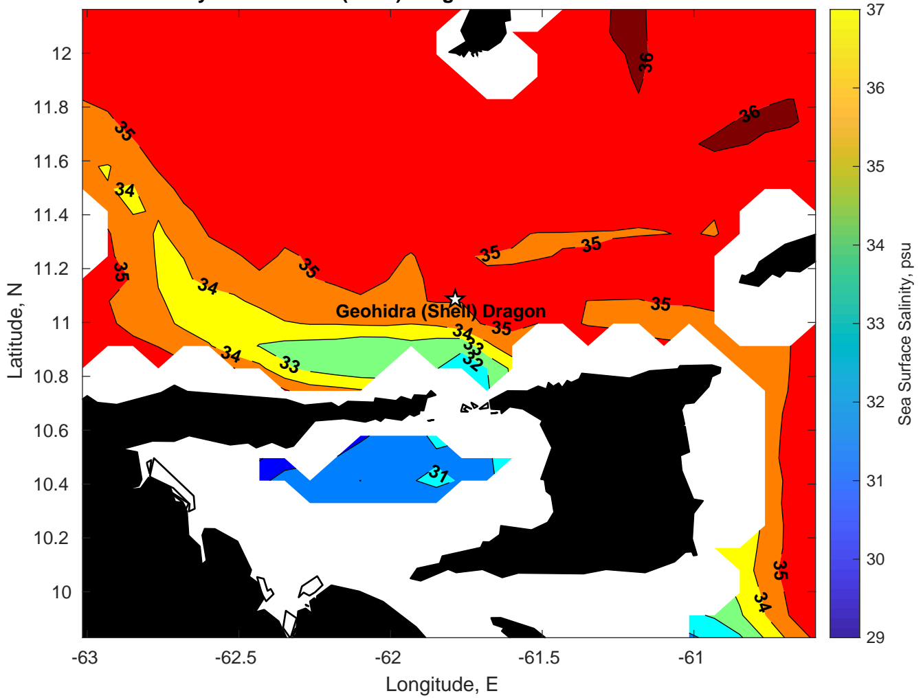
Surface Salinity for Geohidra (Shell) Dragon at 15-Jan-2025 00:00:00
