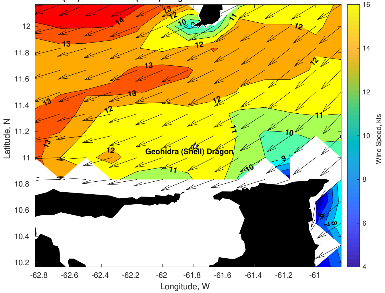
Winds (kts) for Geohidra (Shell) Dragon at 16-Jan-2025 09:00:00
