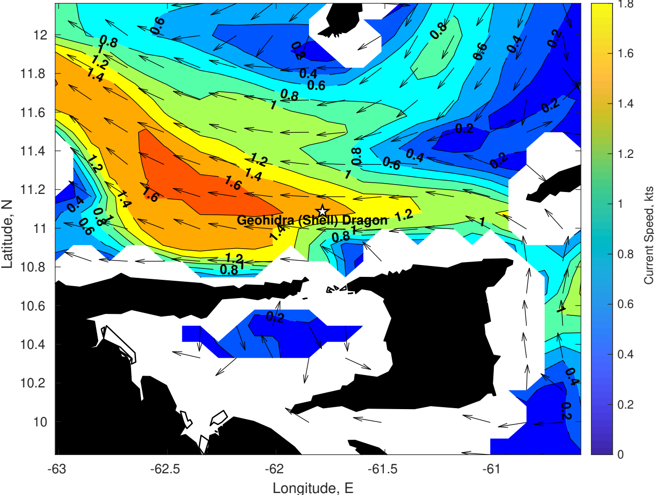
Surface Currents for Geohidra (Shell) Dragon at 15-Jan-2025 00:00:00
