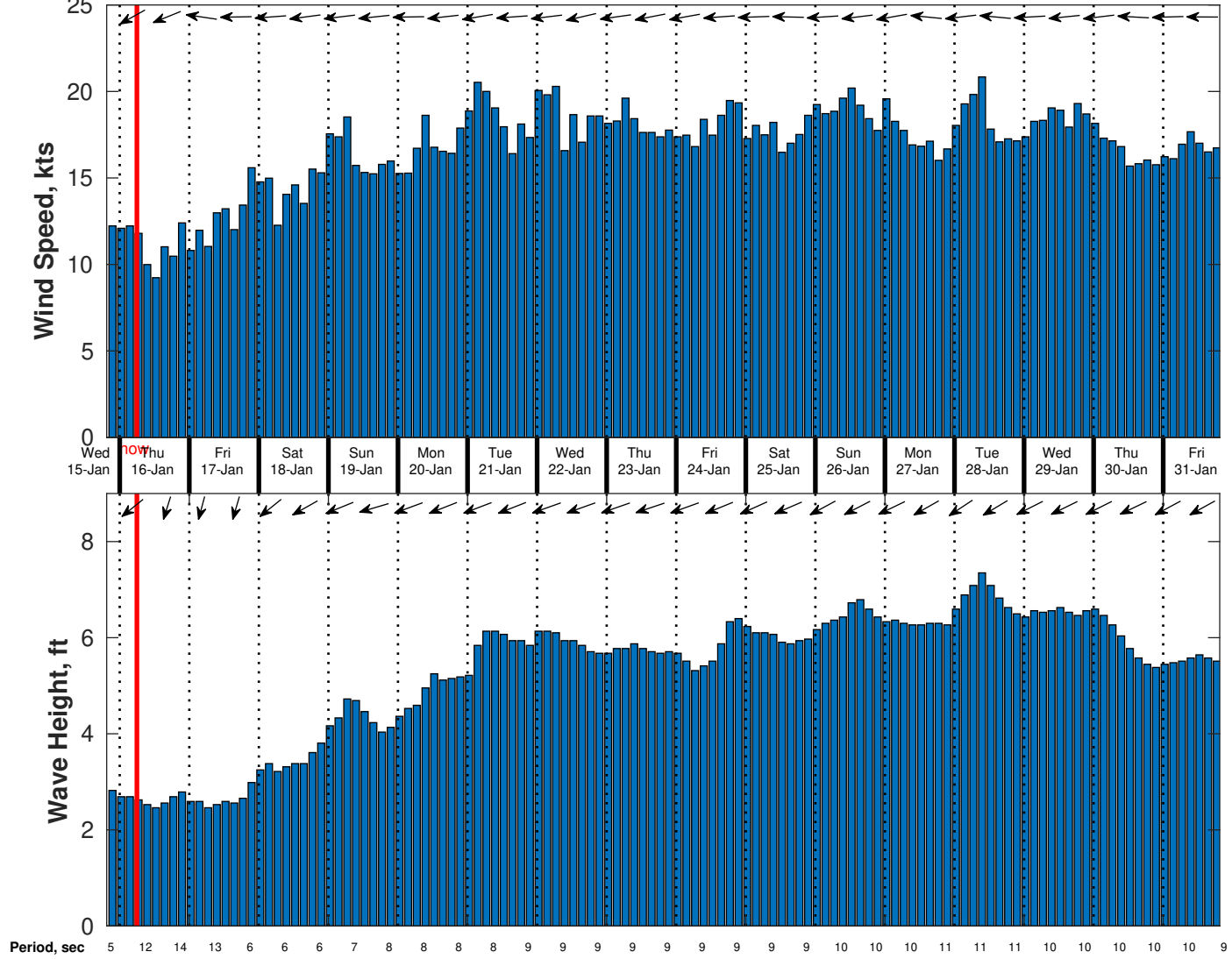
Wind & Wave Forecast for Geohidra (Shell) Dragon from 15-Jan-2025 20:00:00 to 31-Jan-2025 20:00:00
