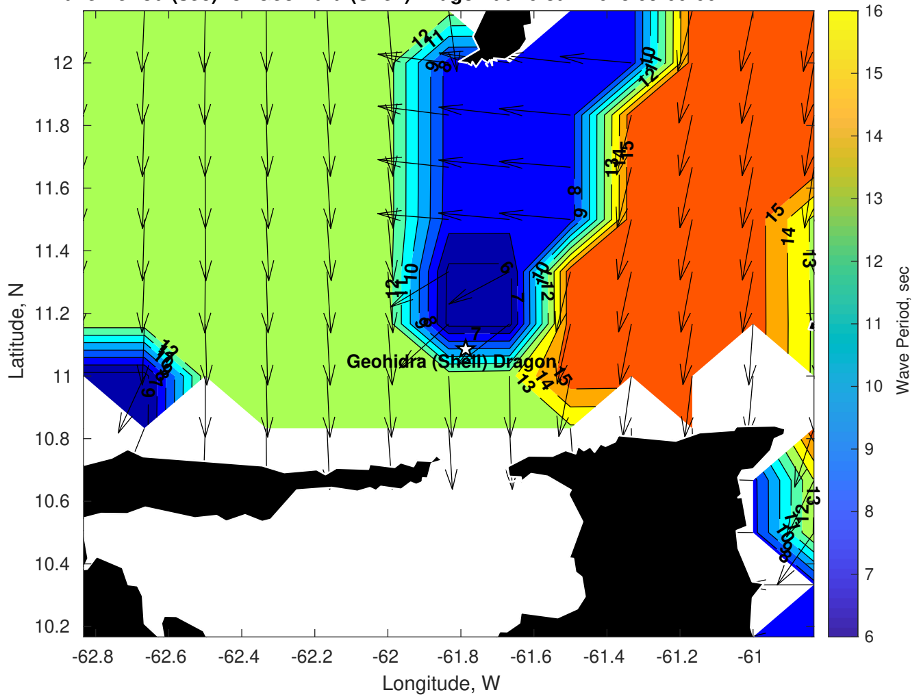
Wave Period (sec) for Geohidra (Shell) Dragon at 16-Jan-2025 09:00:00
