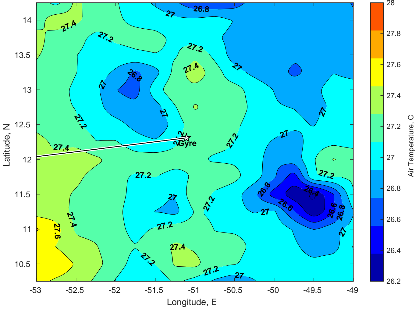
Air Temperature (C) for Gyre at 16-Jan-2025
