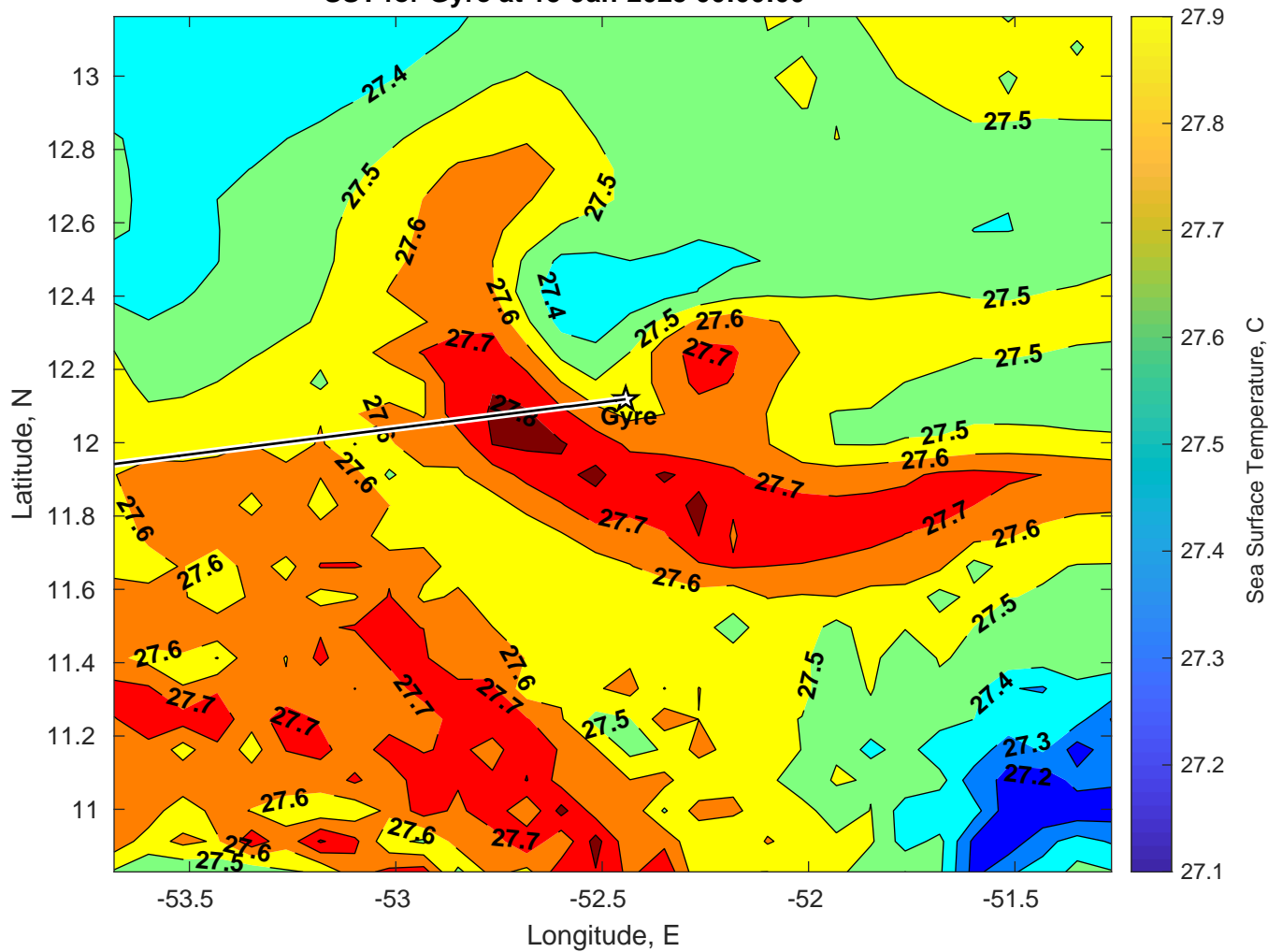
SST for Gyre at 15-Jan-2025 00:00:00
