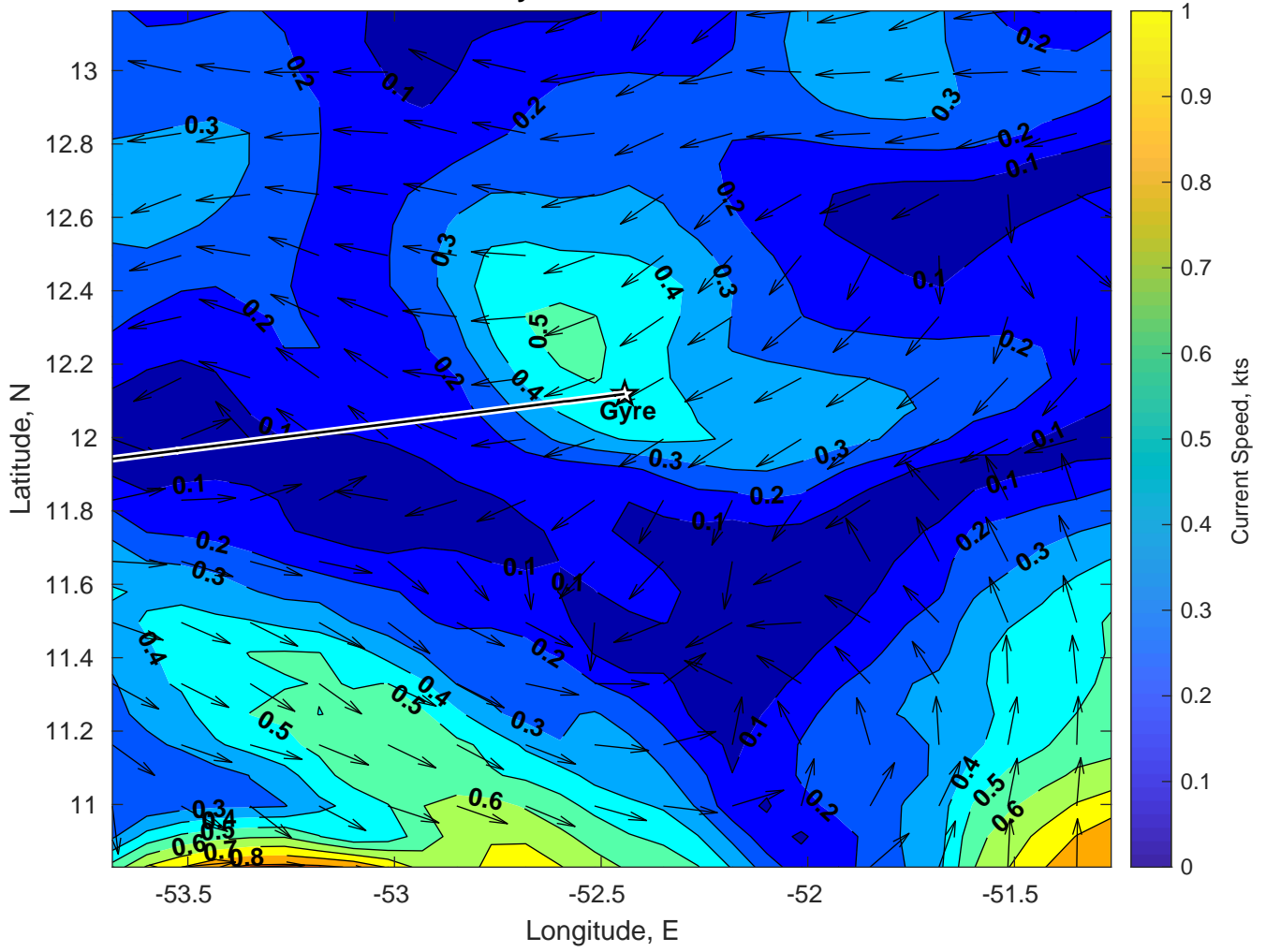
Surface Currents for Gyre at 15-Jan-2025 00:00:00
