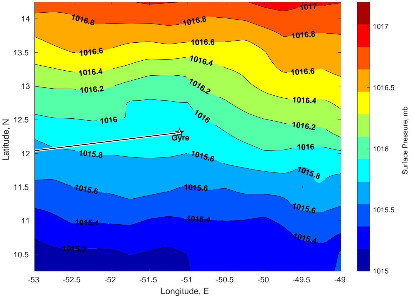
Surface Pressure (mb) for Gyre at 18-Jan-2025 00:00:00
