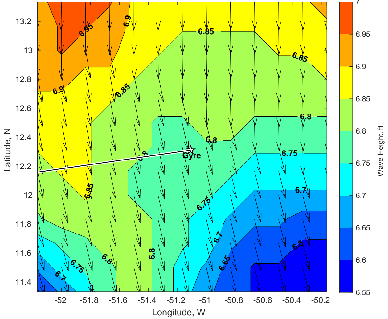
Wave Height (ft) for Gyre at 16-Jan-2025 09:00:00
