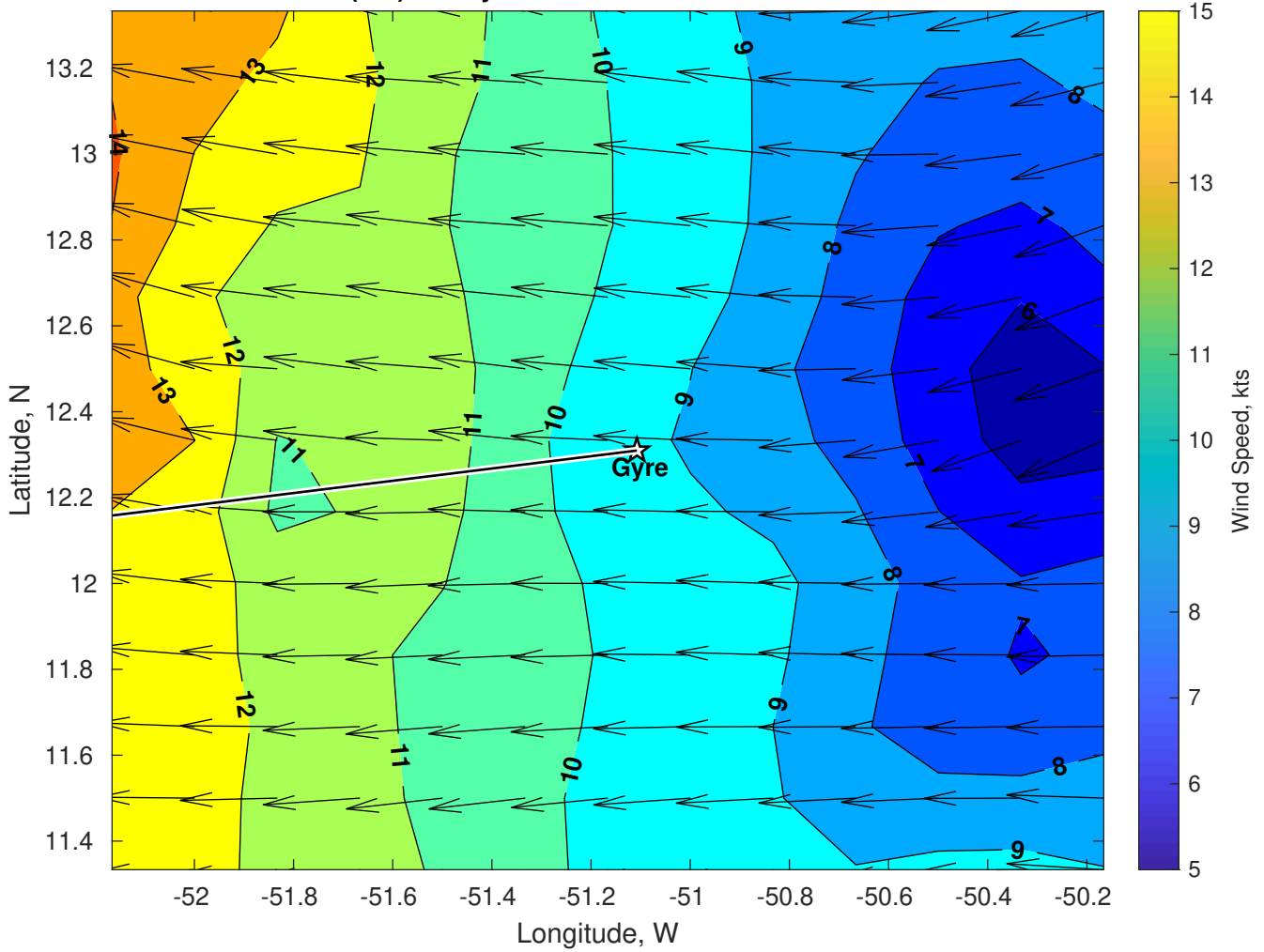
Winds (kts) for Gyre at 16-Jan-2025 09:00:00
