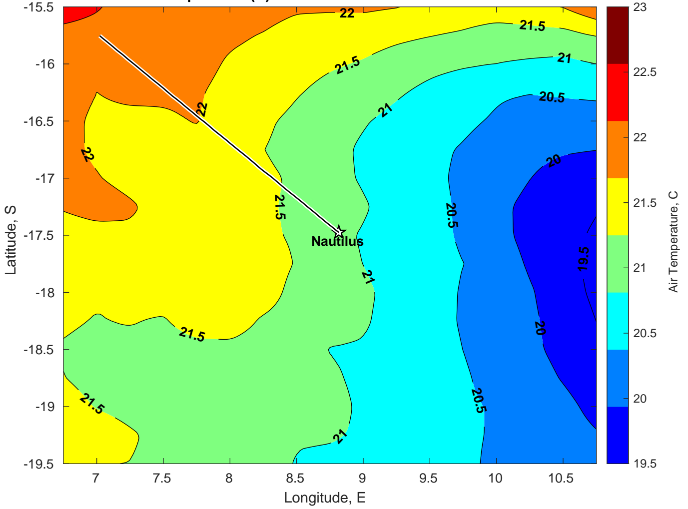
Air Temperature (C) for Nautilus at 16-Jan-2025
