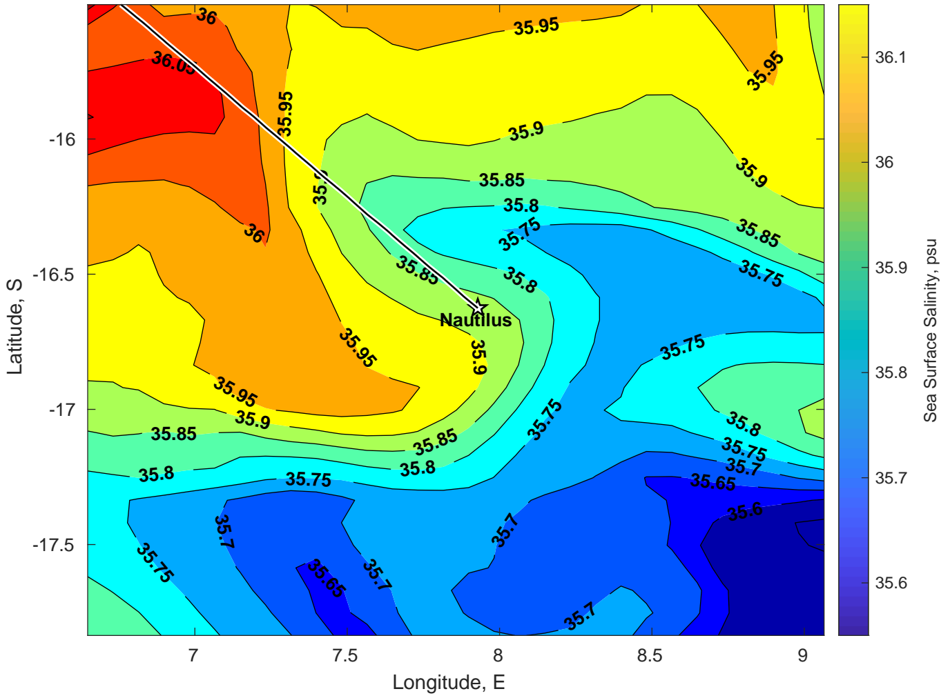
Surface Salinity for Nautilus at 15-Jan-2025 00:00:00
