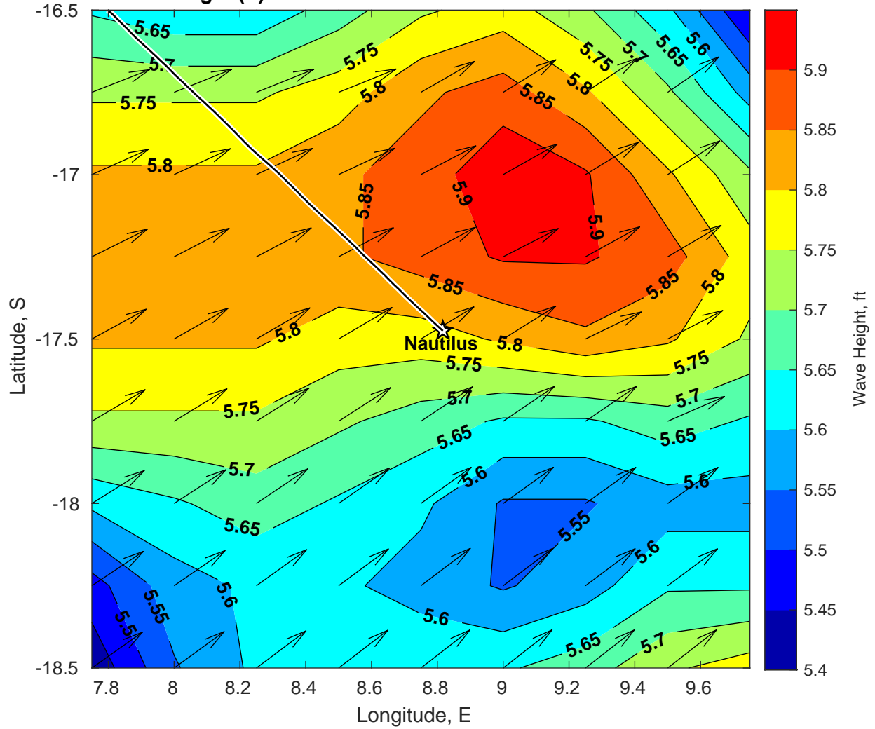
Wave Height (ft) for Nautilus at 16-Jan-2025 09:00:00
