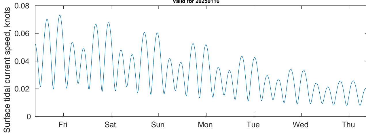
Tidal Currents and Heights for Nautilus at 20250116
