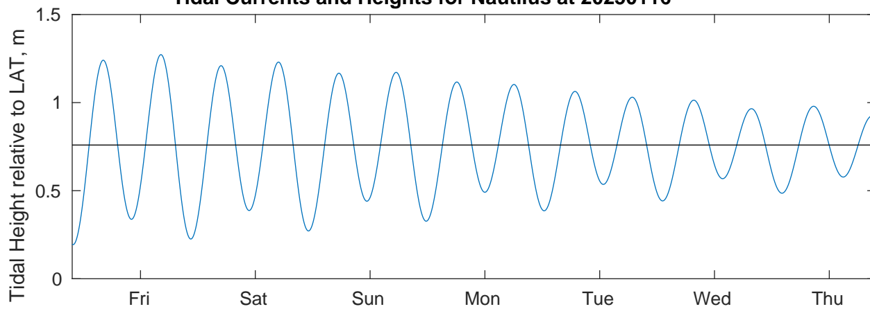
Tidal Currents and Heights for Nautilus at 20250116
