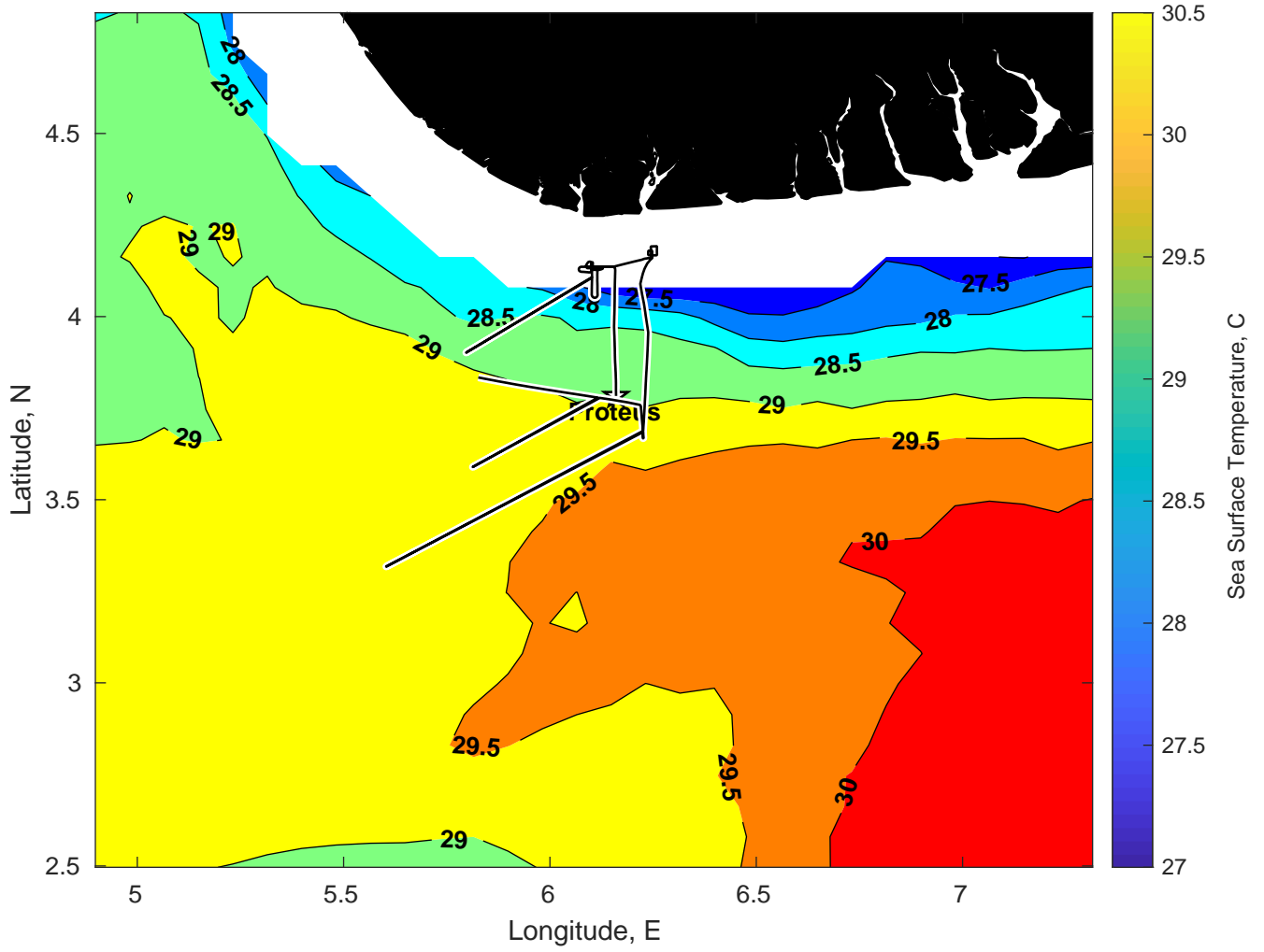
SST for Proteus at 15-Jan-2025 00:00:00
