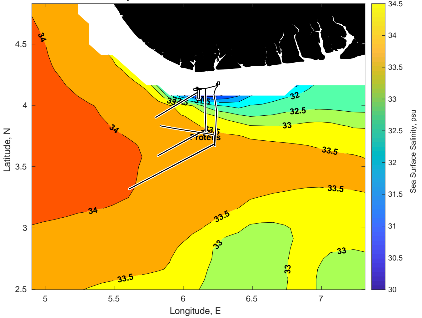
Surface Salinity for Proteus at 15-Jan-2025 00:00:00
