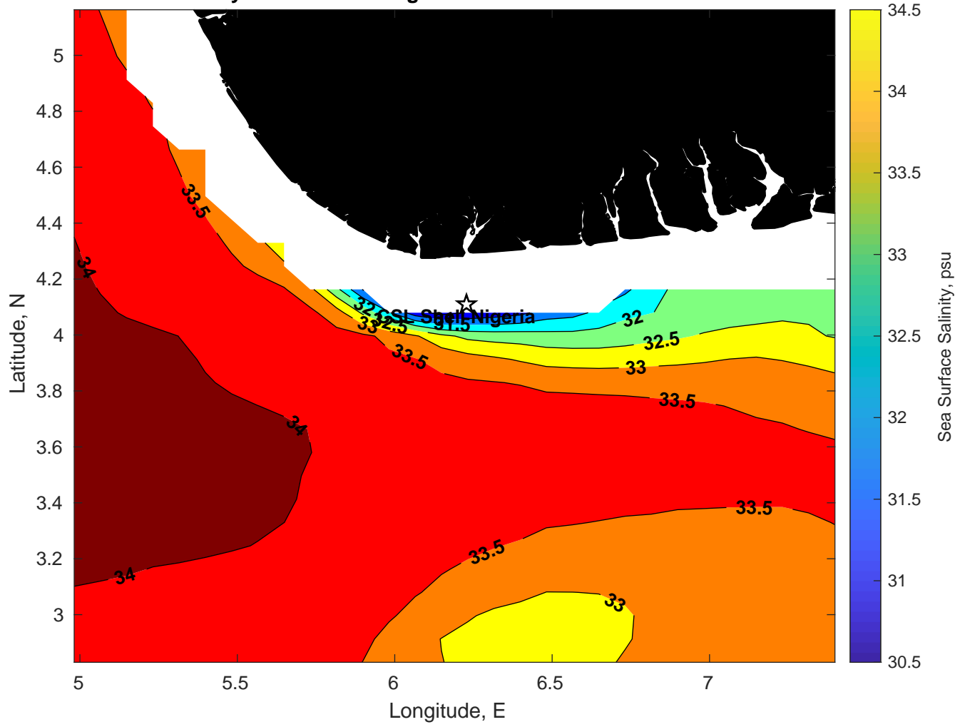
Surface Salinity for CSL Shell Nigeria at 16-Jan-2025 00:00:00
