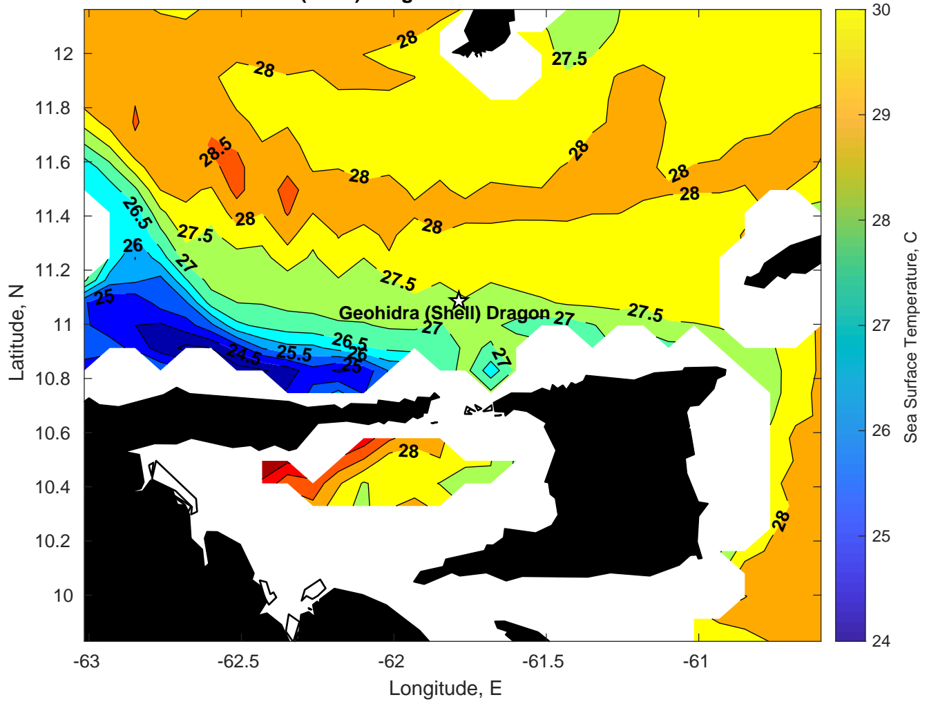
SST for Geohidra (Shell) Dragon at 16-Jan-2025 00:00:00
