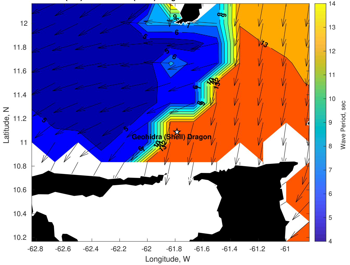
Wave Period (sec) for Geohidra (Shell) Dragon at 17-Jan-2025 09:00:00
