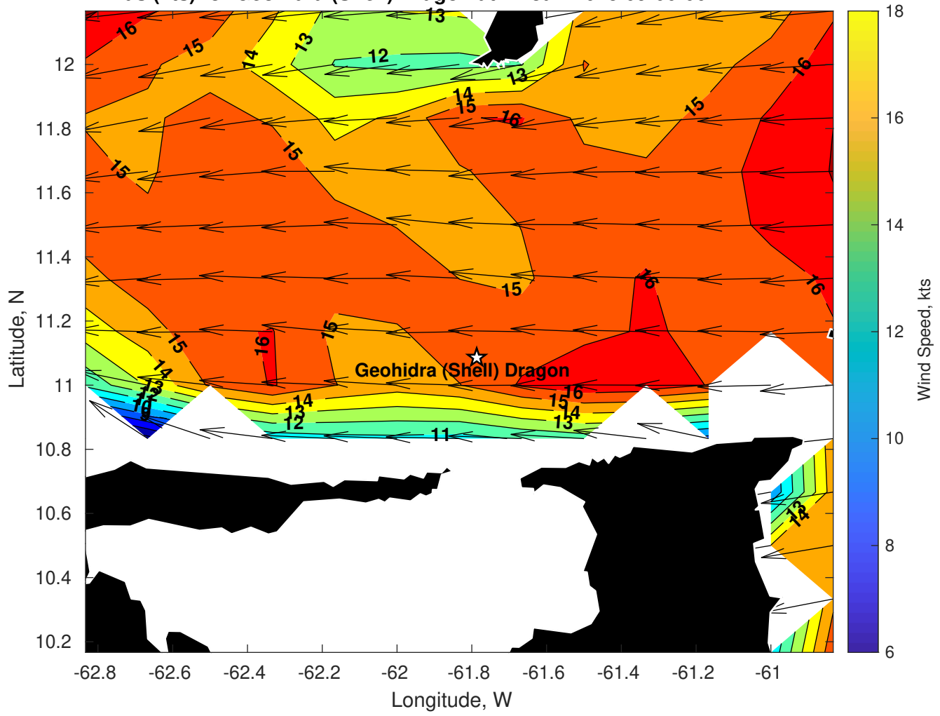
Winds (kts) for Geohidra (Shell) Dragon at 17-Jan-2025 09:00:00
