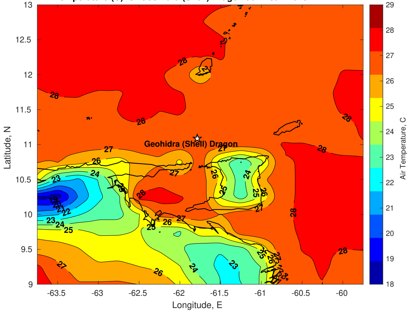
Air Temperature (C) for Geohidra (Shell) Dragon at 17-Jan-2025
