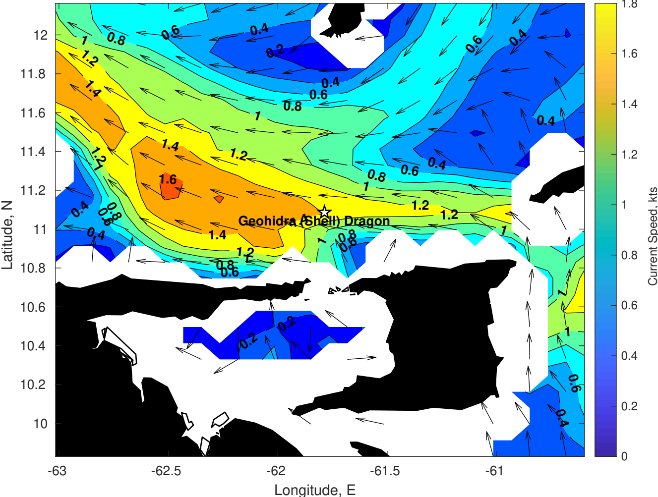
Surface Currents for Geohidra (Shell) Dragon at 16-Jan-2025 00:00:00
