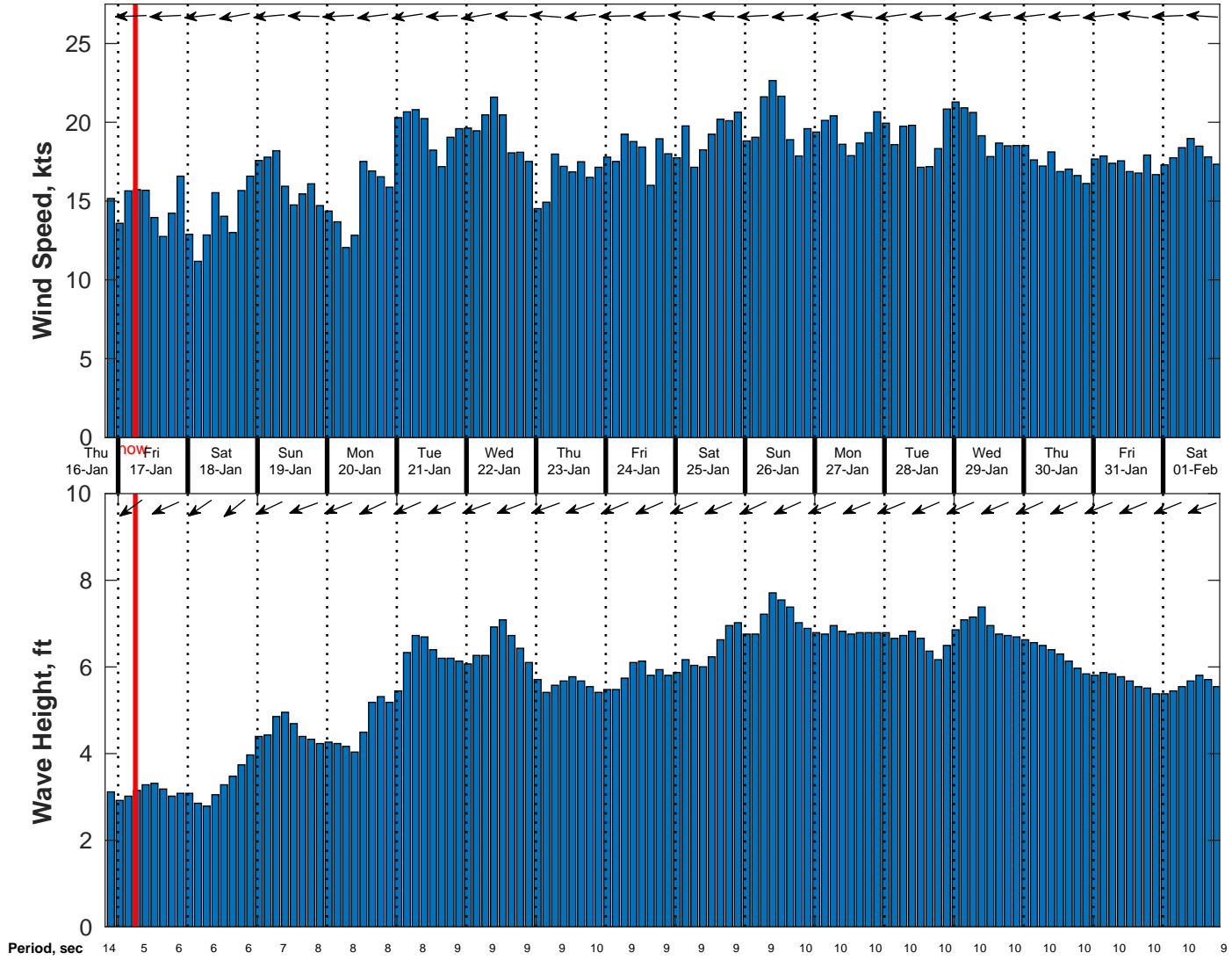
Wind & Wave Forecast for Geohira (Shell) Dragon from 16-Jan-2025 20:00:00 to 01-Feb-2025 20:00:00
