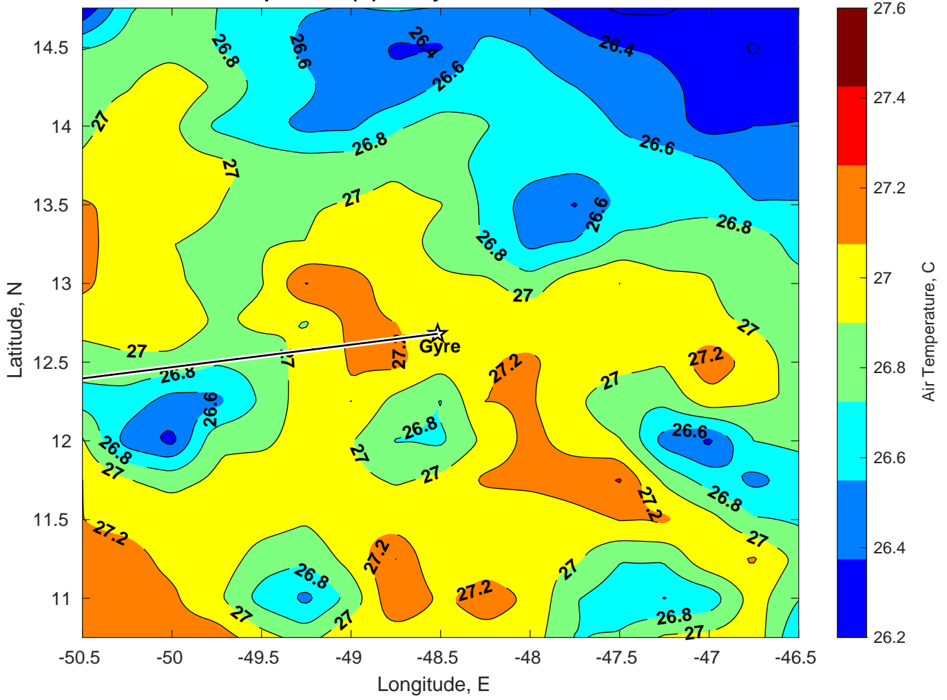
Air Temperature (C) for Gyre at 17-Jan-2025
