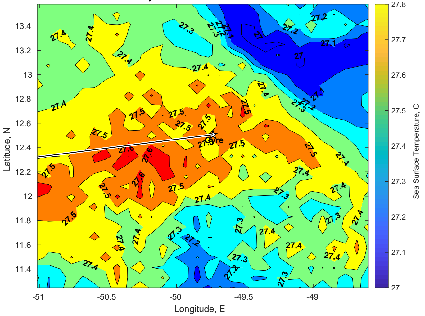
SST for Gyre at 16-Jan-2025 00:00:00
